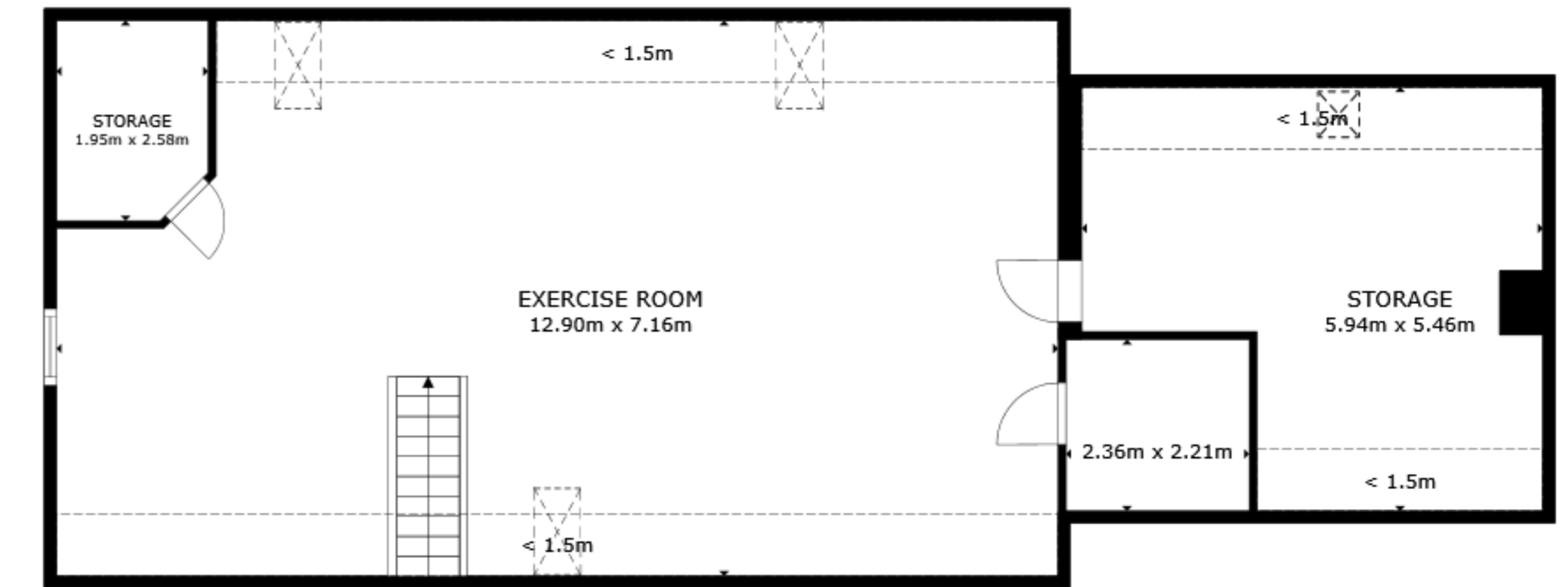
FLOOR 3
