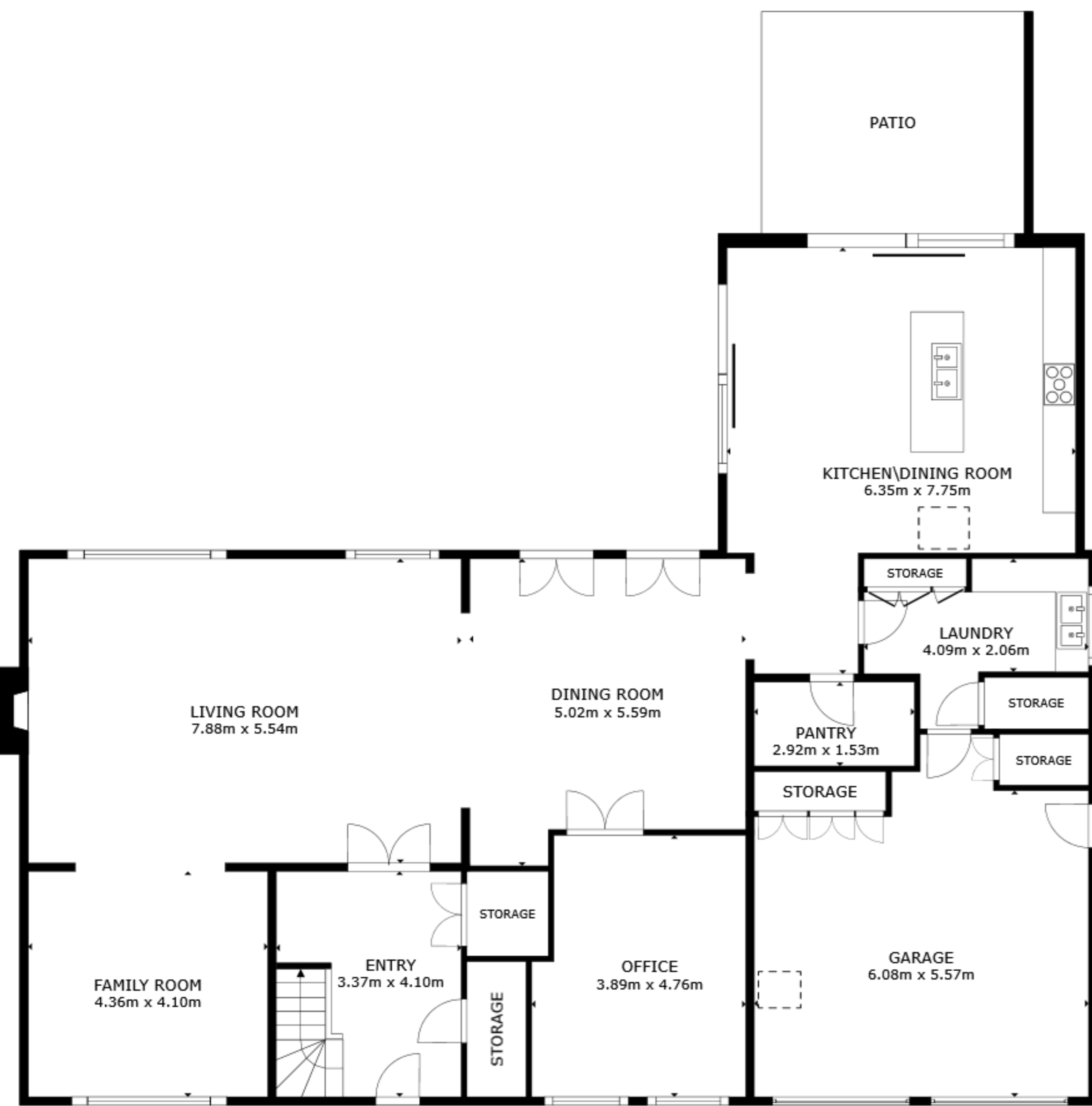
FLOOR 1
