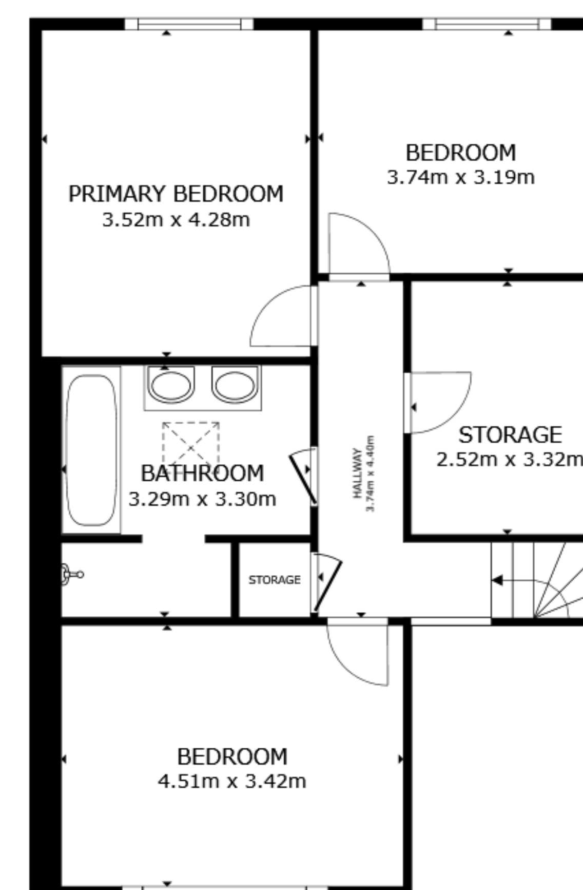
FLOOR 2
