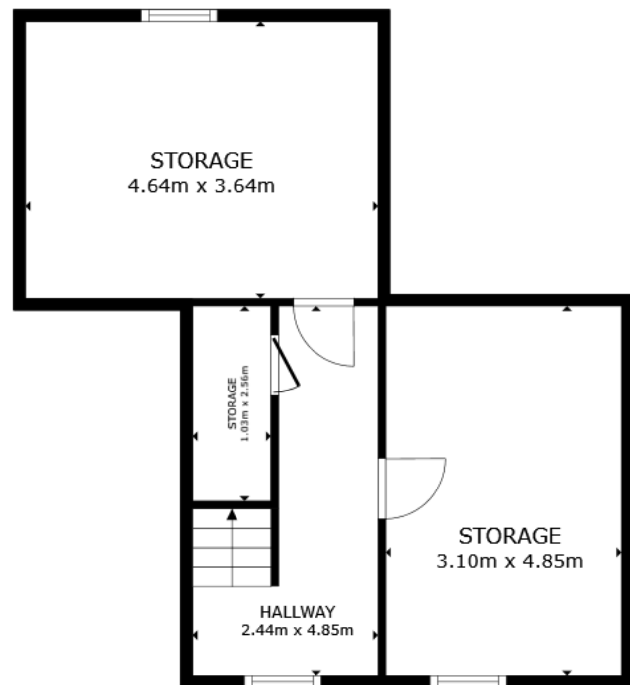
FLOOR 1
