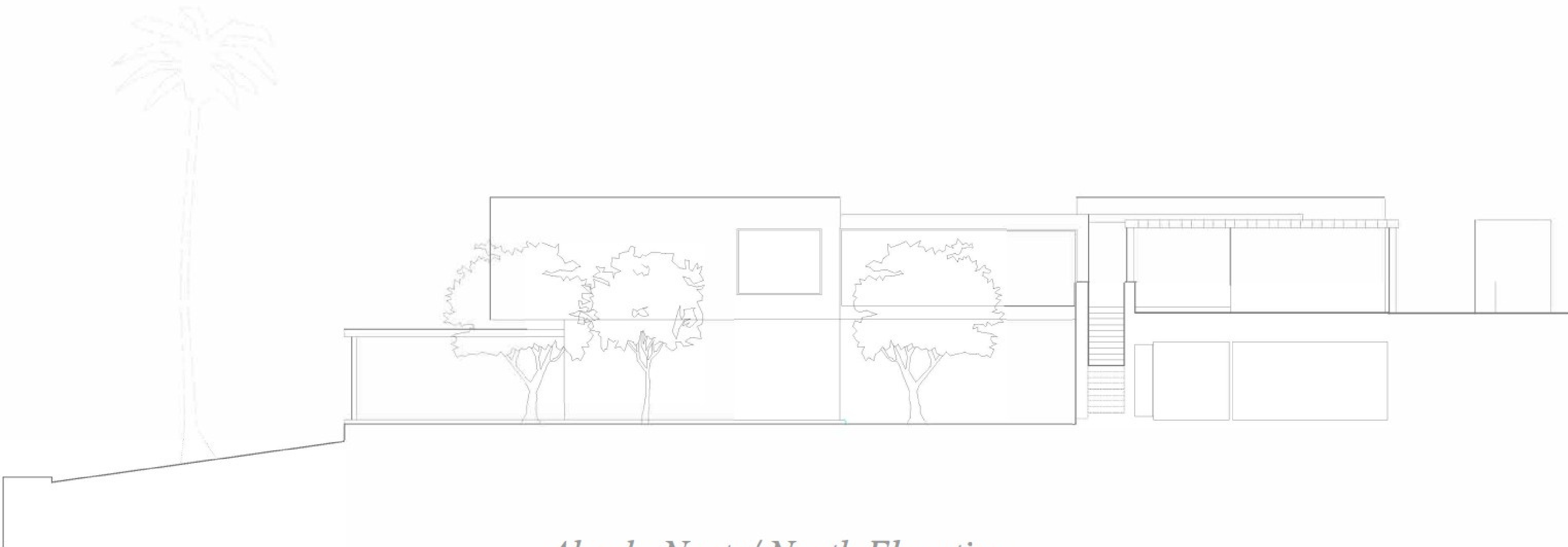
Alzado Norte/ North Elevation
