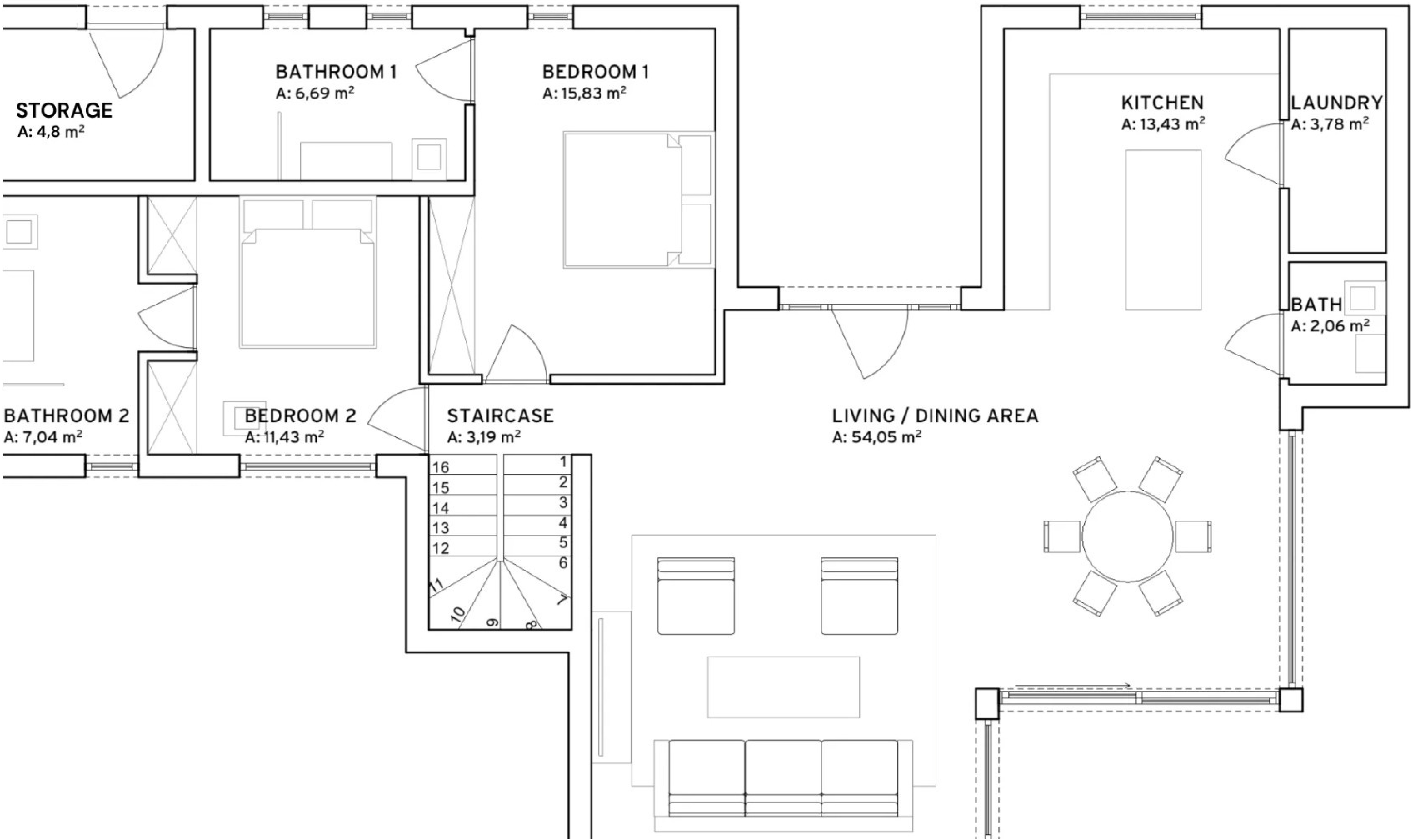
JORPLAN GROUND FLOOR 1:100
