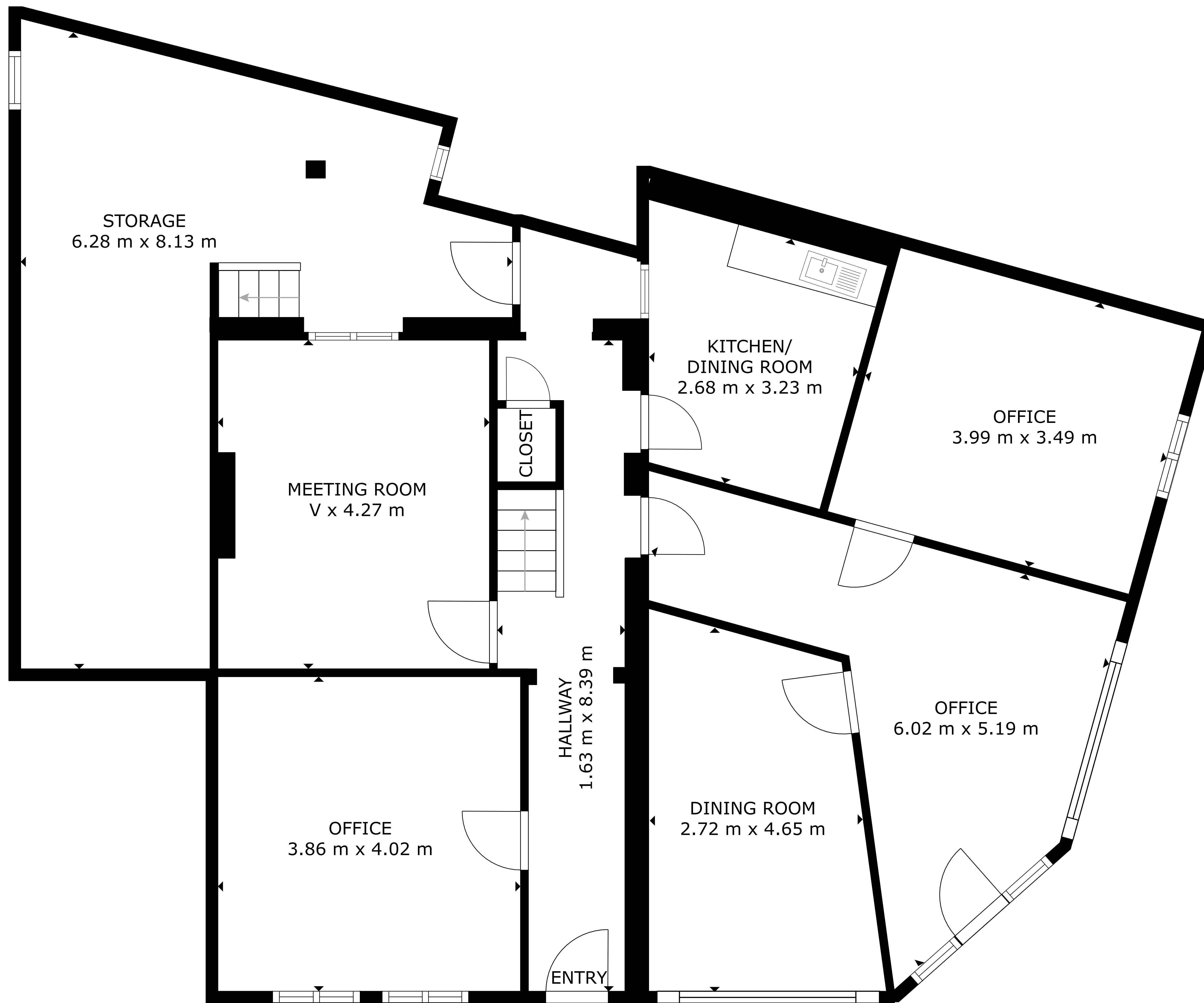
FLOOR 1
