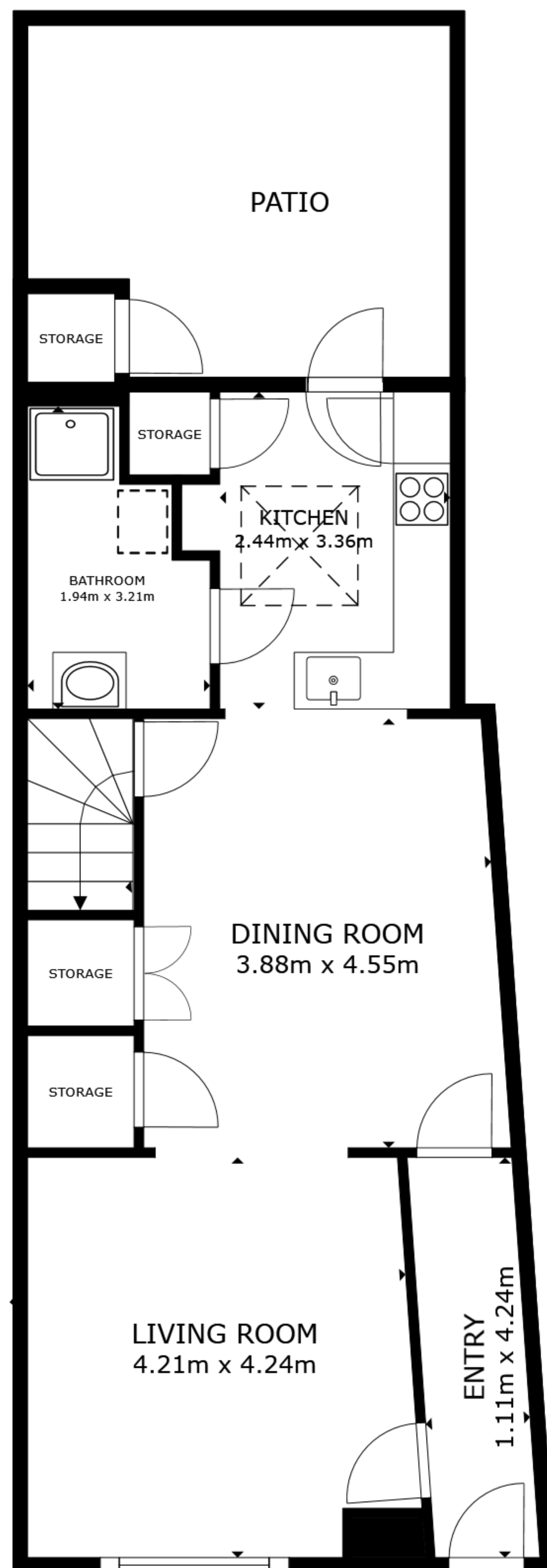
FLOOR 1
