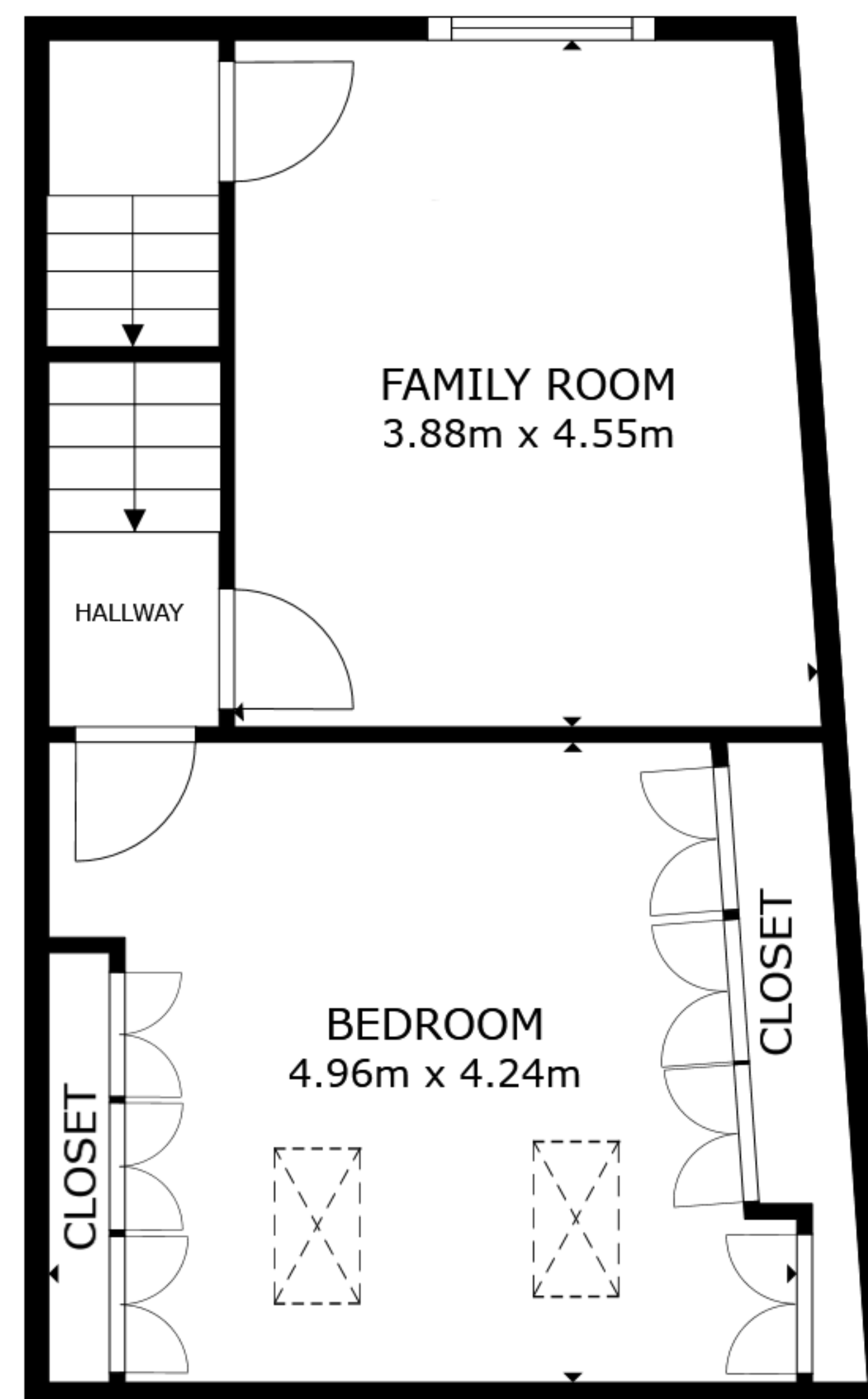
FLOOR 2
