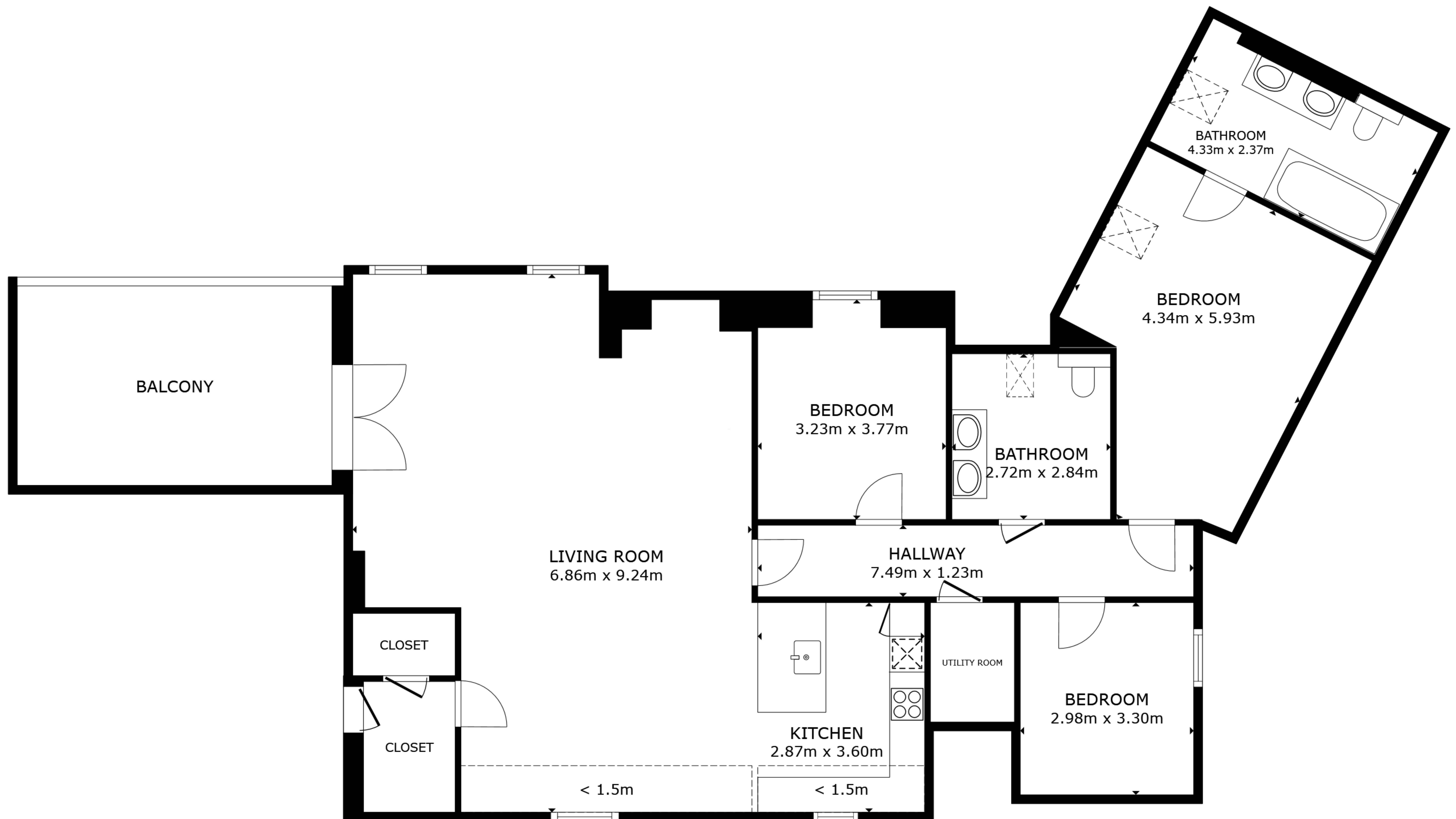
FLOOR PLAN
