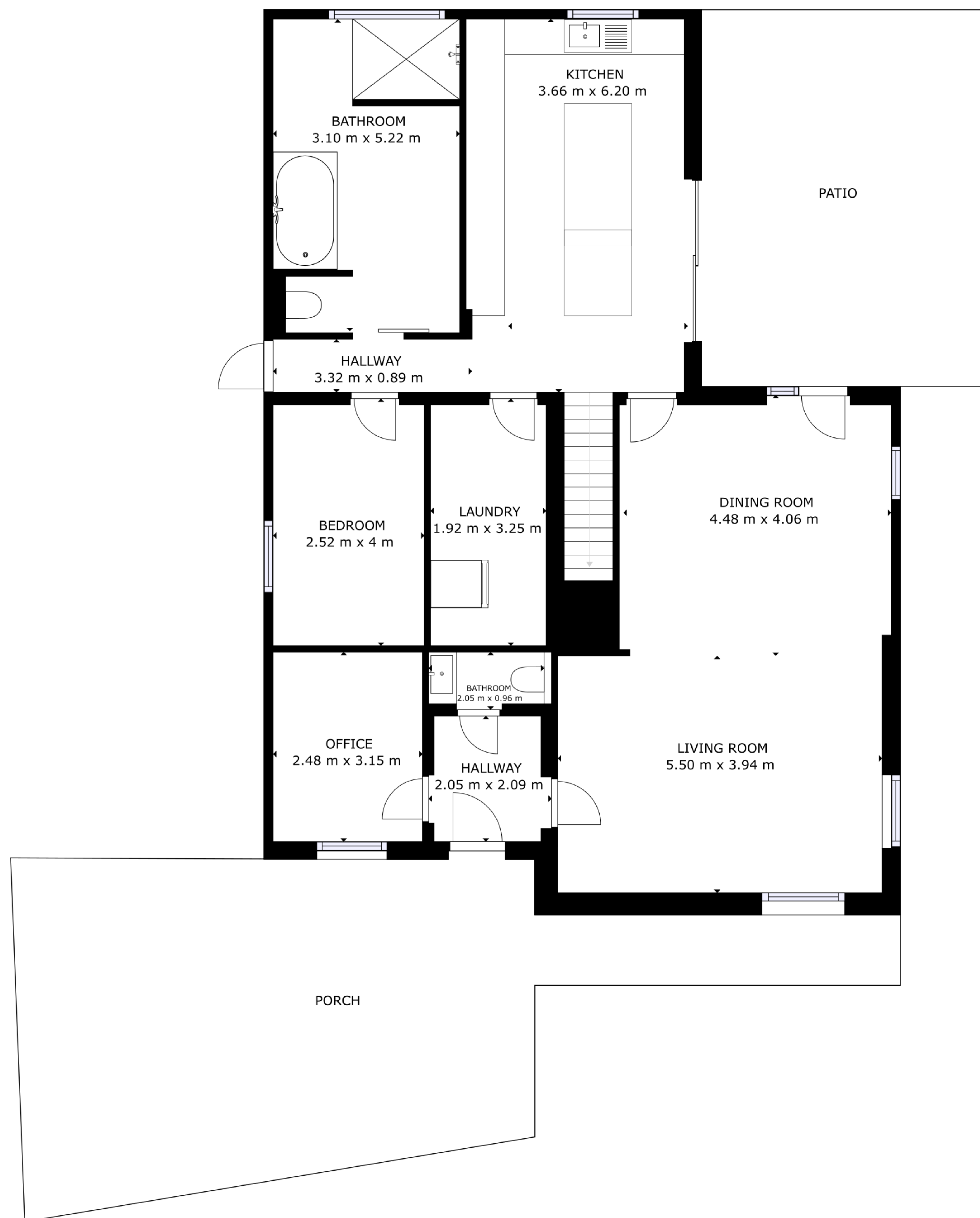
FLOOR 1
