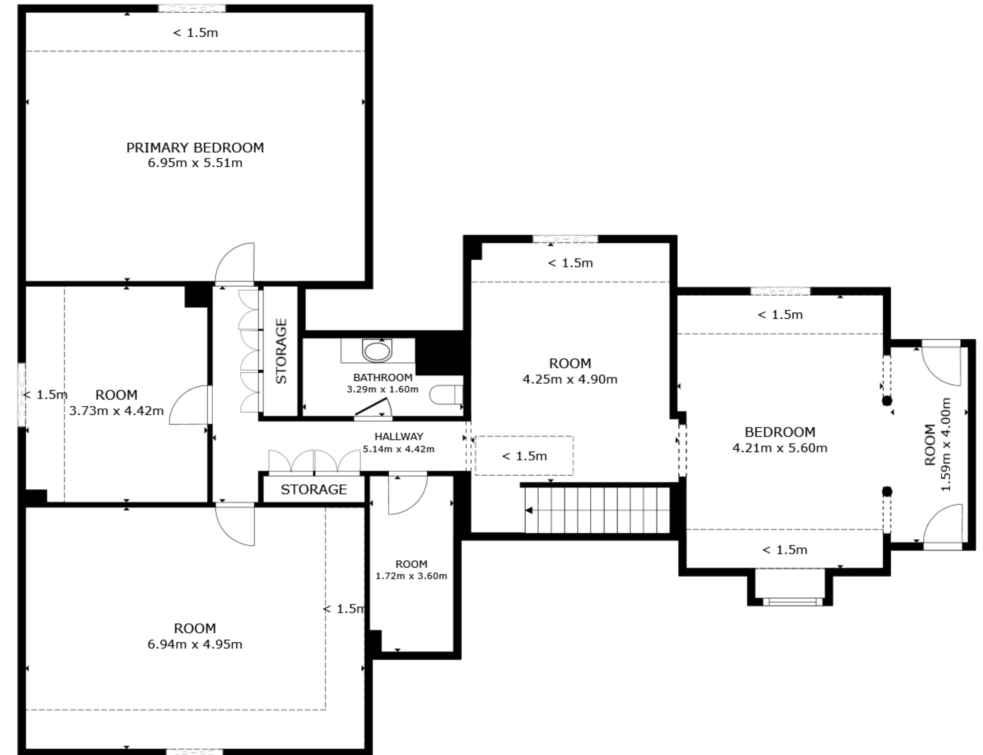
FLOOR 1
