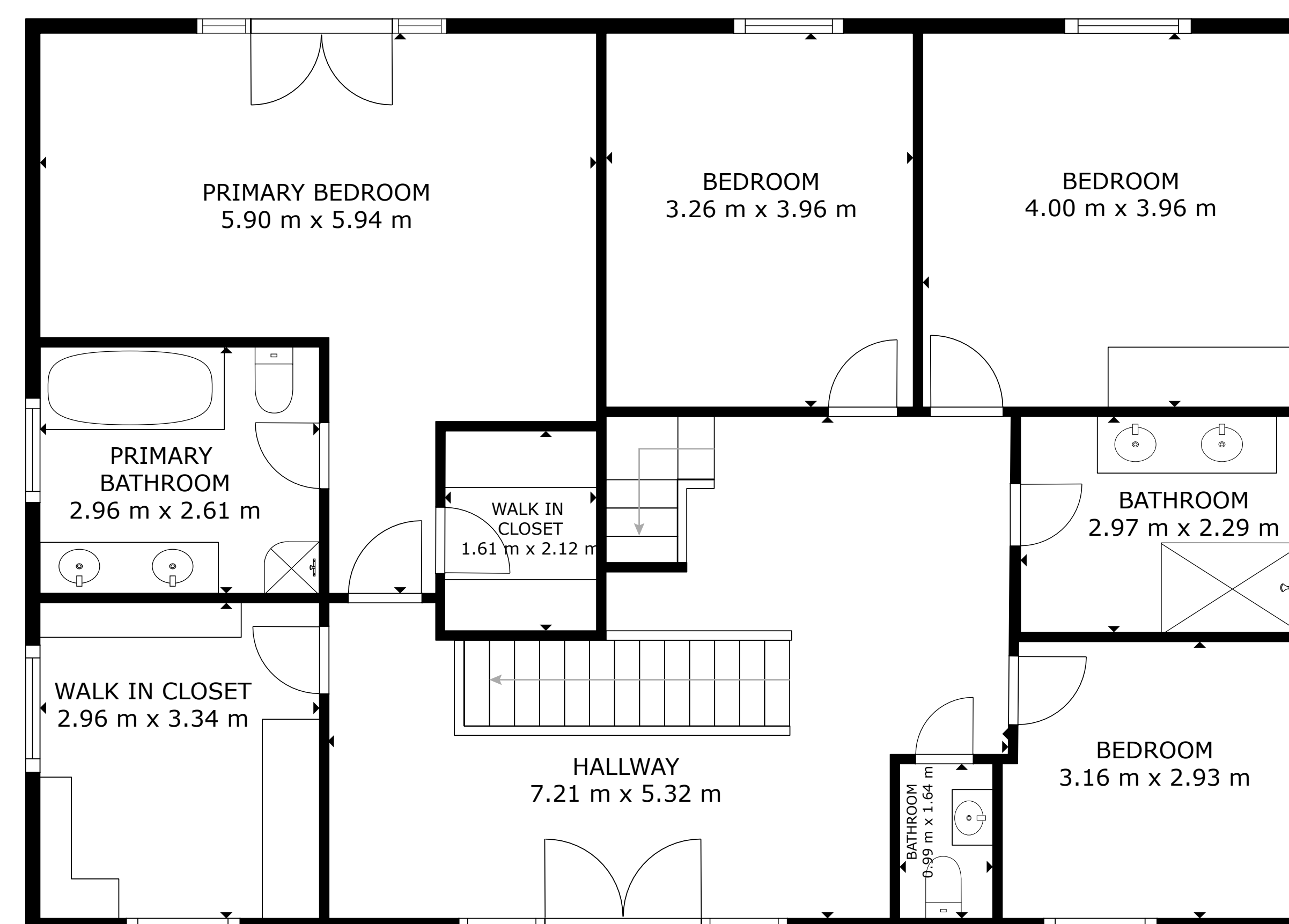
FLOOR 2
