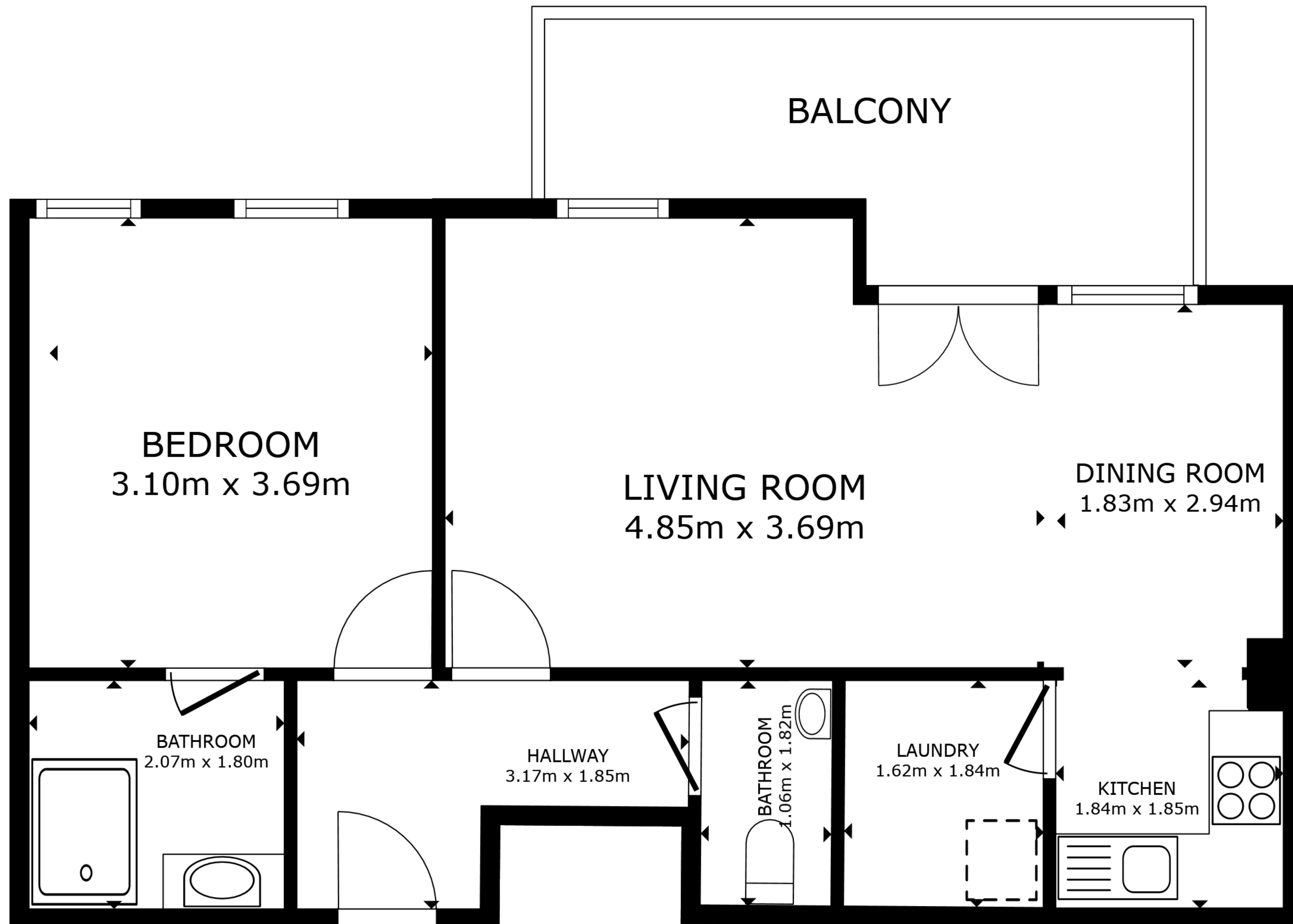
FLOOR PLAN
