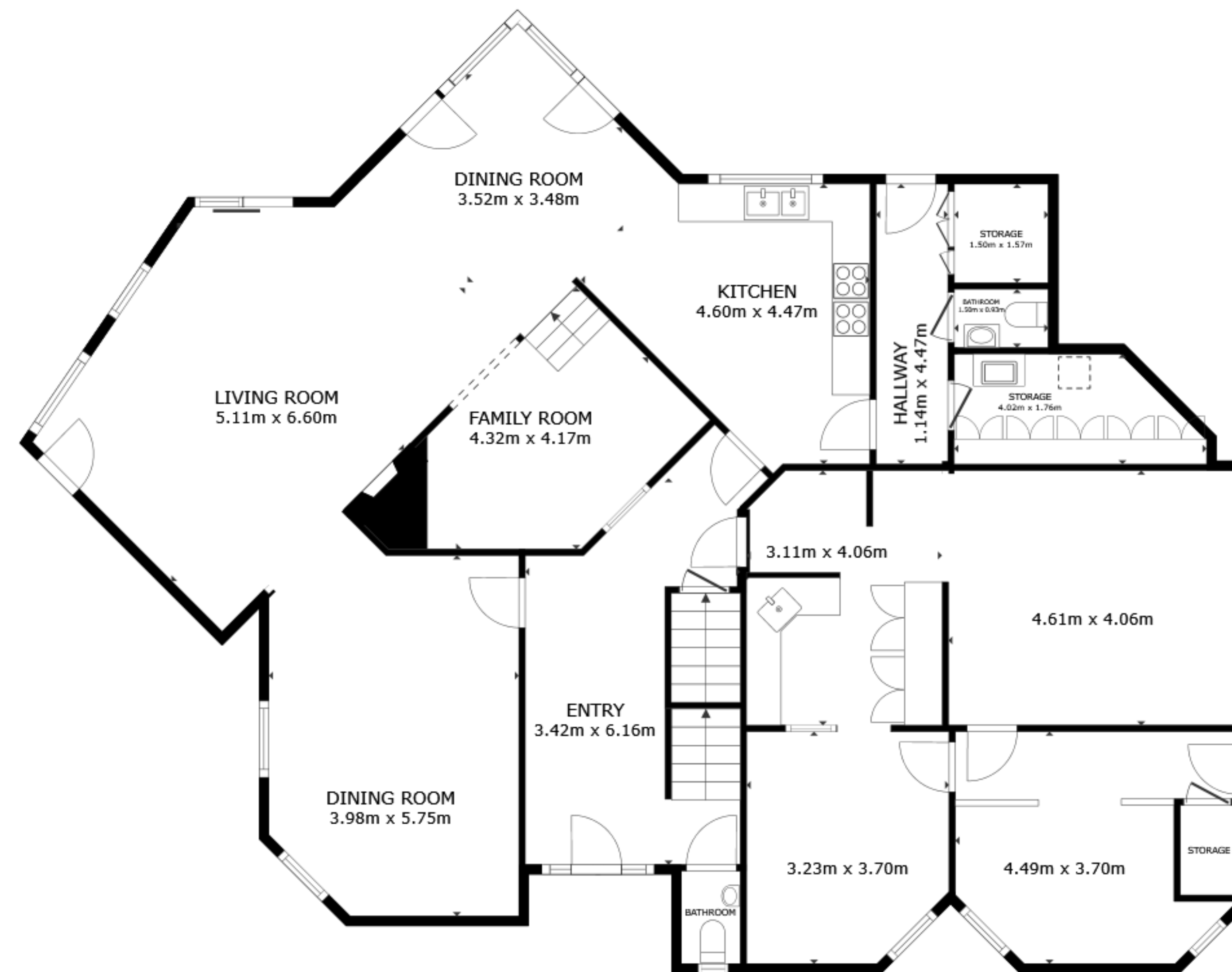
FLOOR 2
