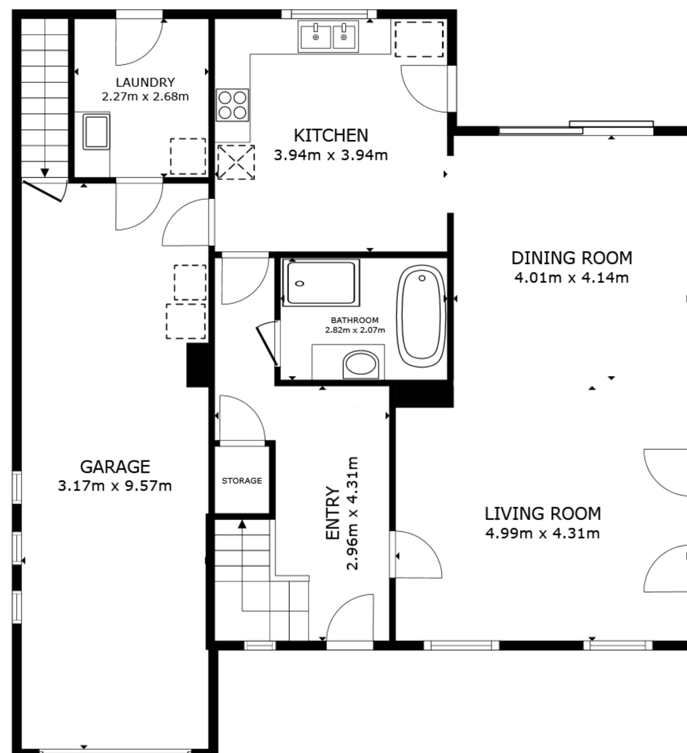
FLOOR 2
