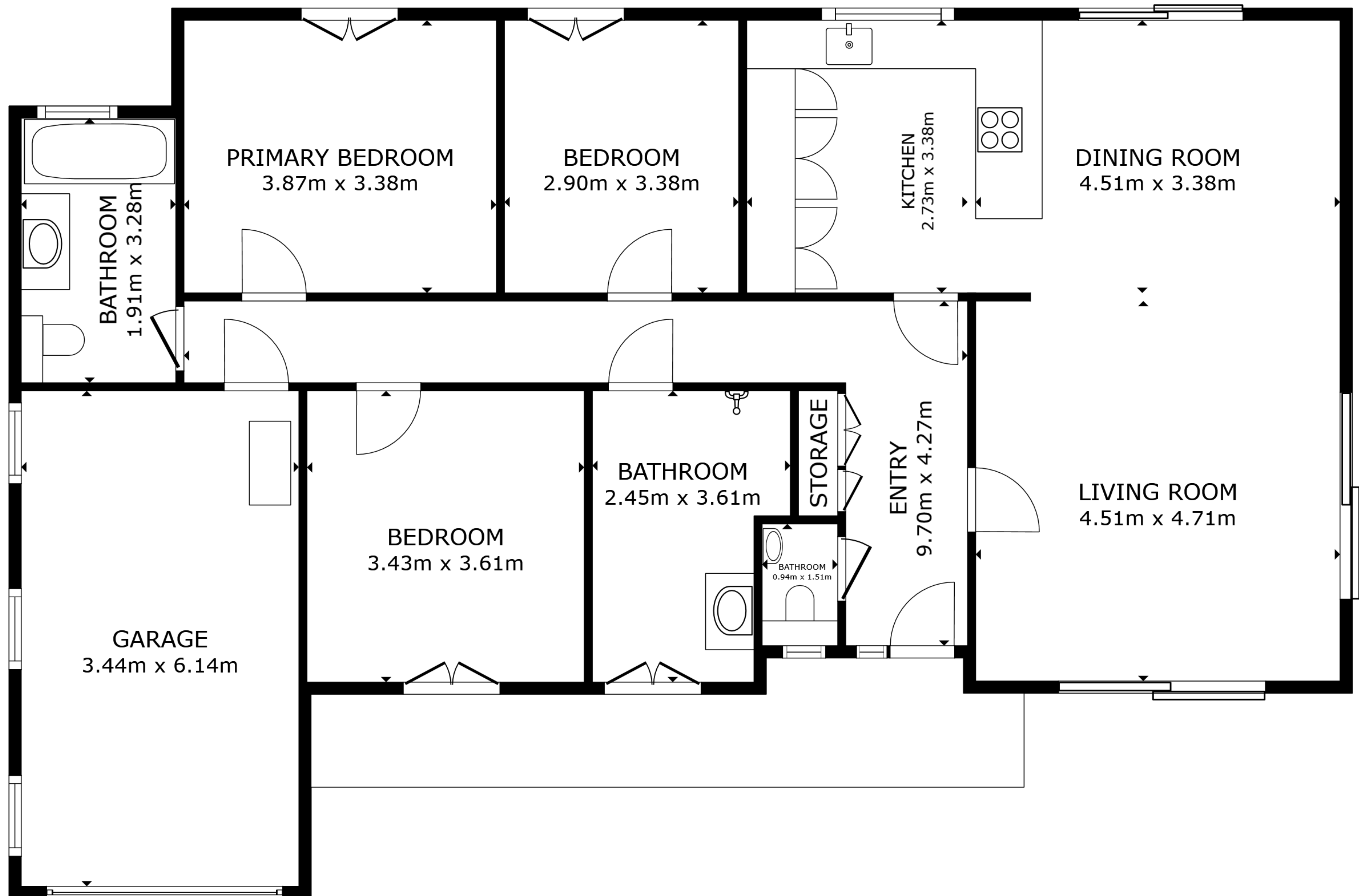
FLOOR PLAN
