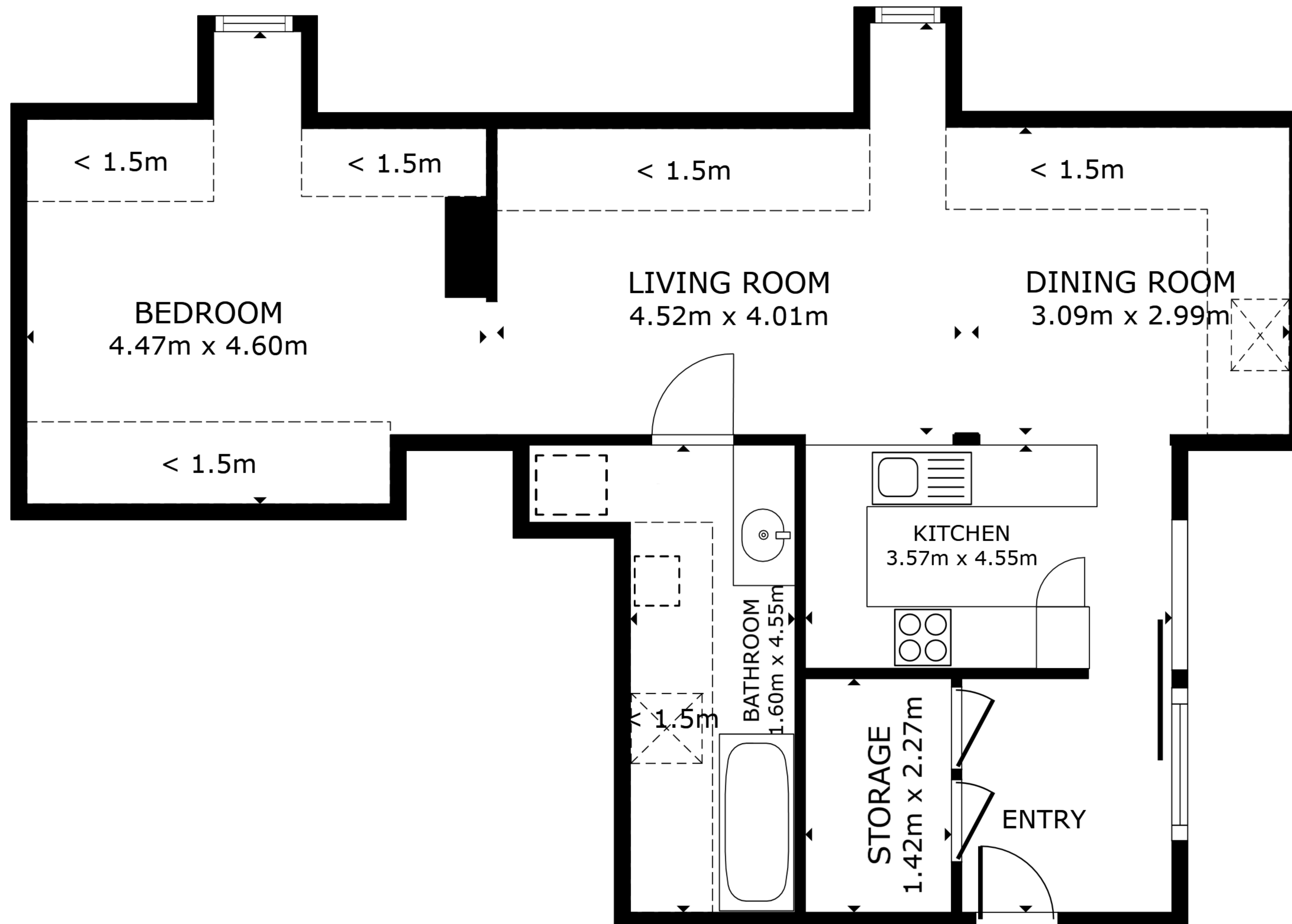
FLOOR PLAN
