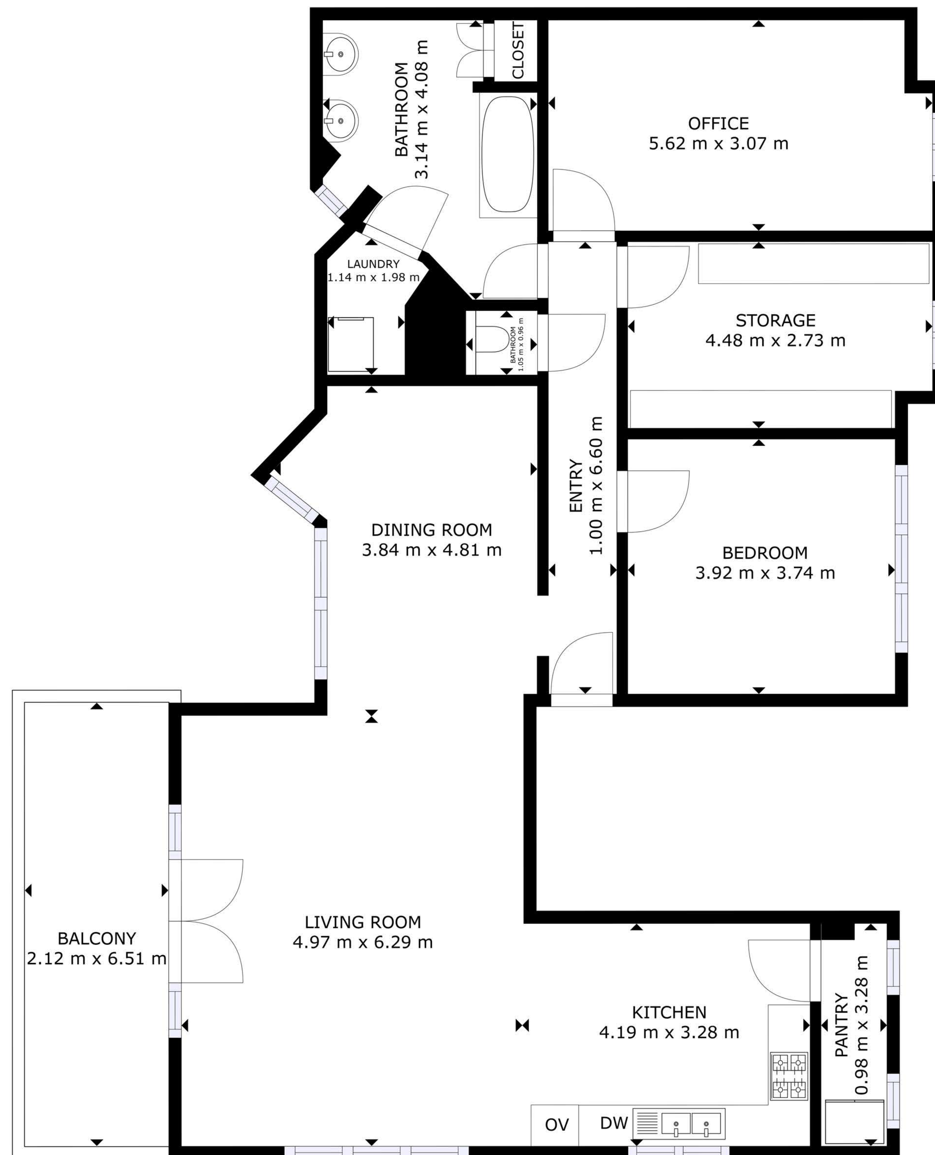
FLOOR PLAN
