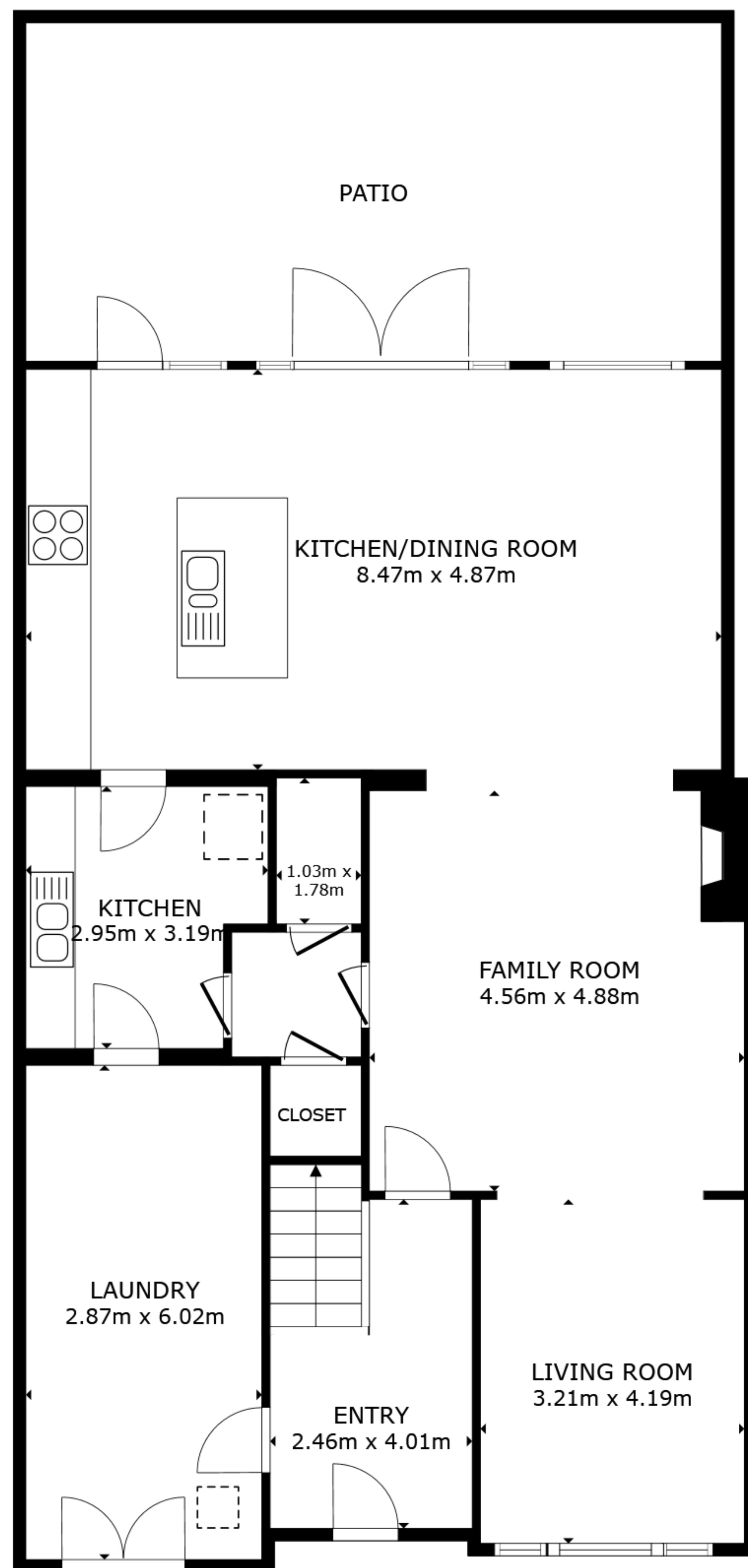
FLOOR 1
