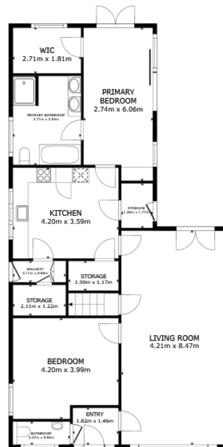
FLOOR 1
