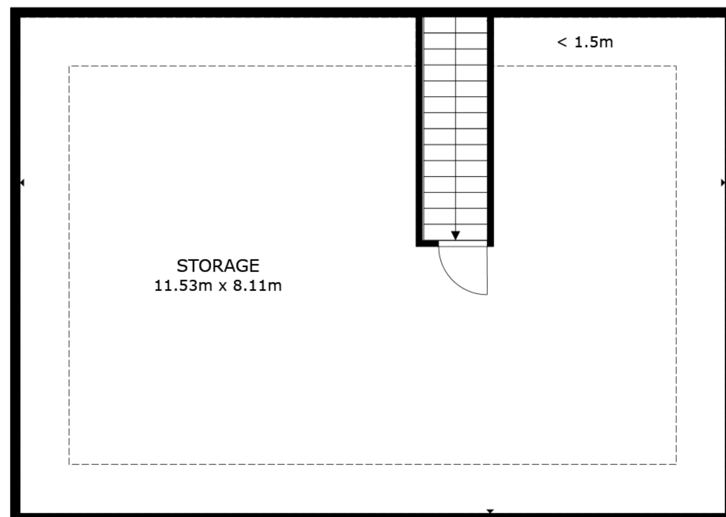
FLOOR 3
