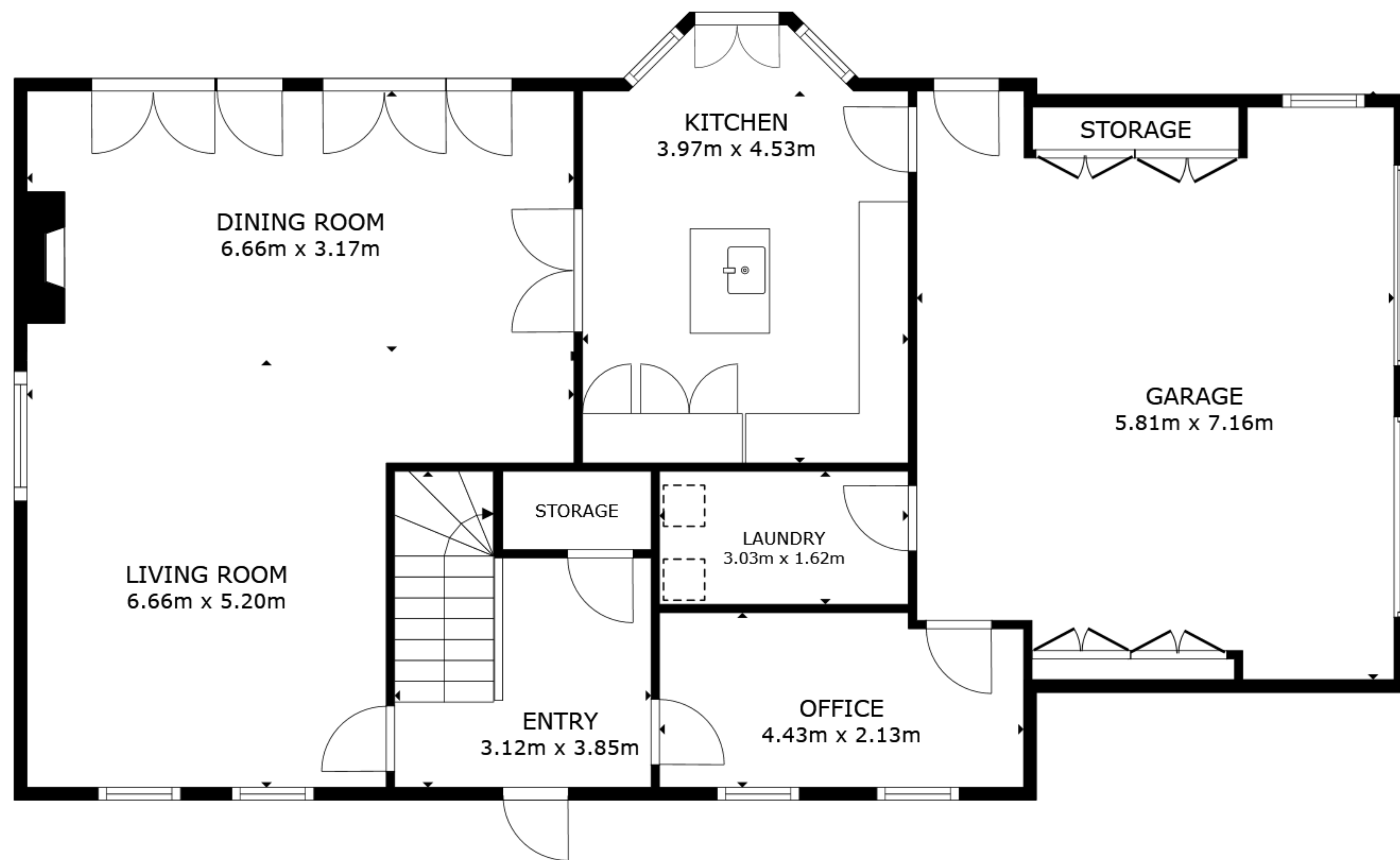
FLOOR 1
