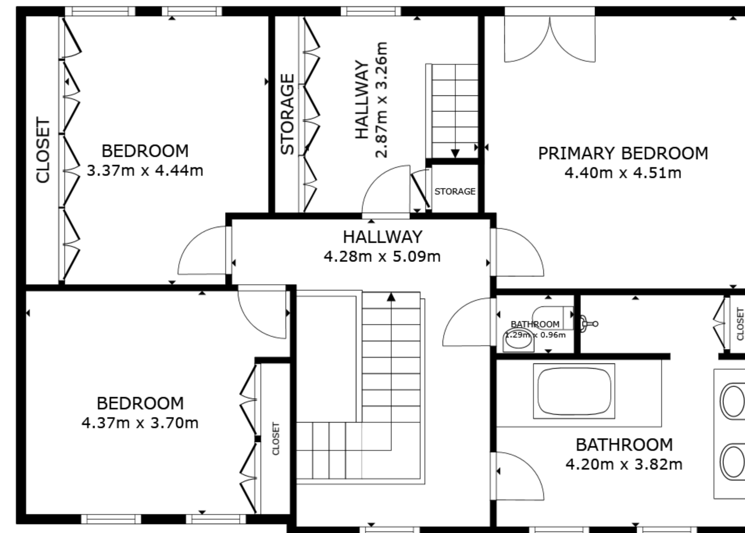
FLOOR 2
