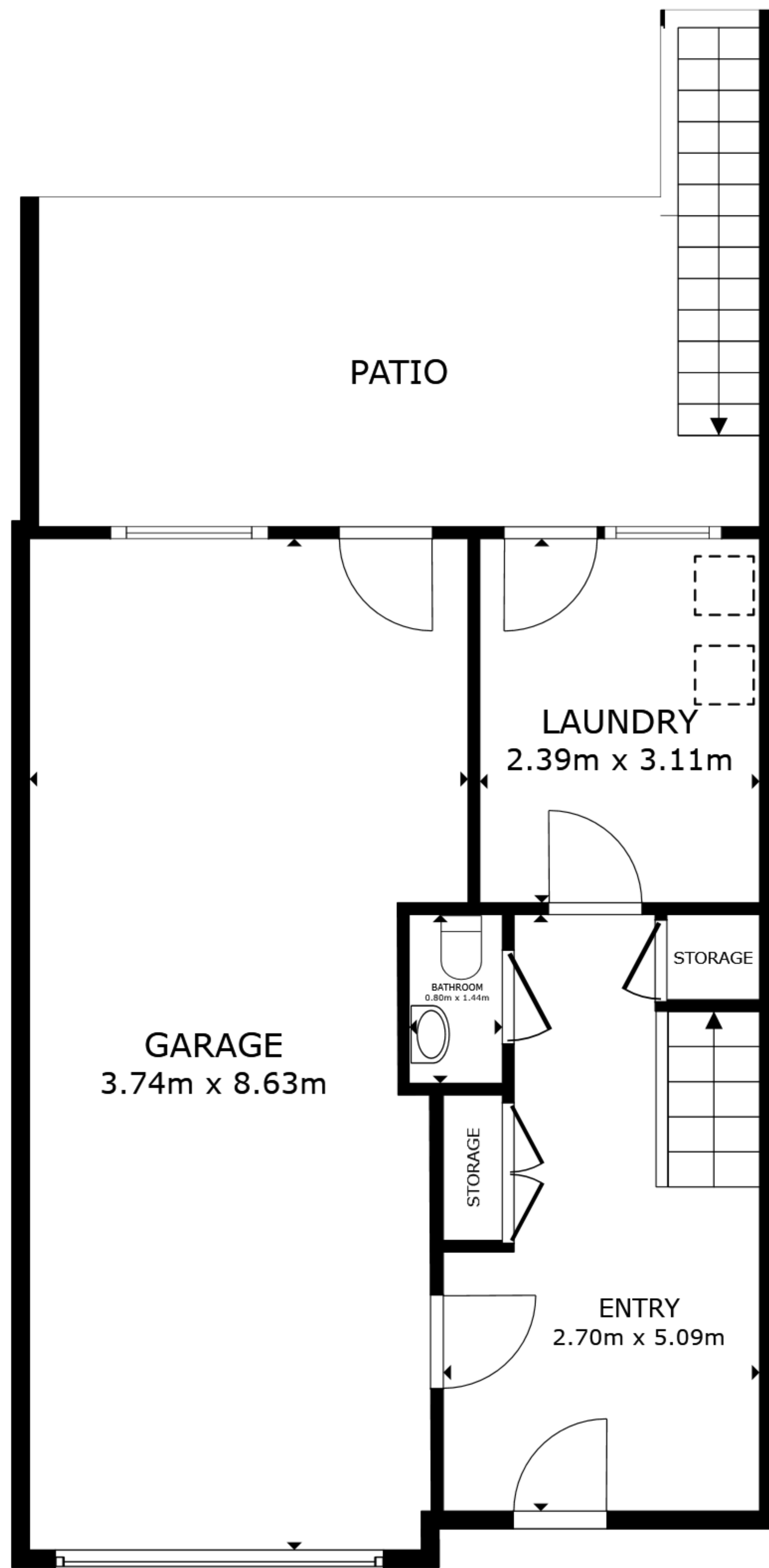
FLOOR 1
