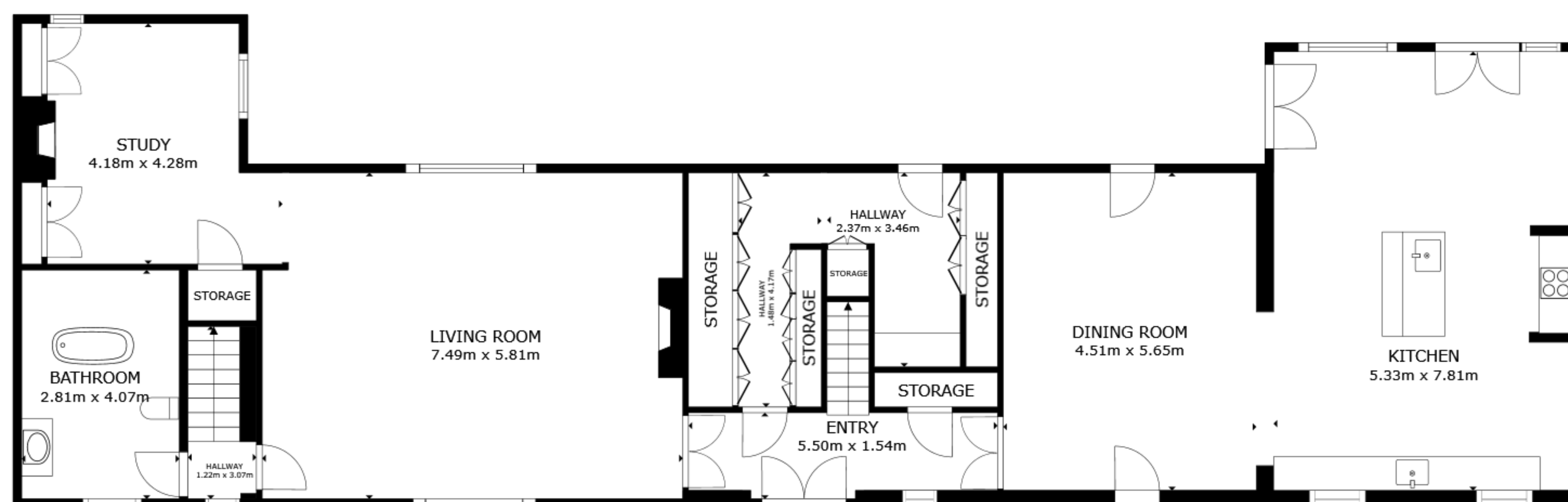
FLOOR 1
