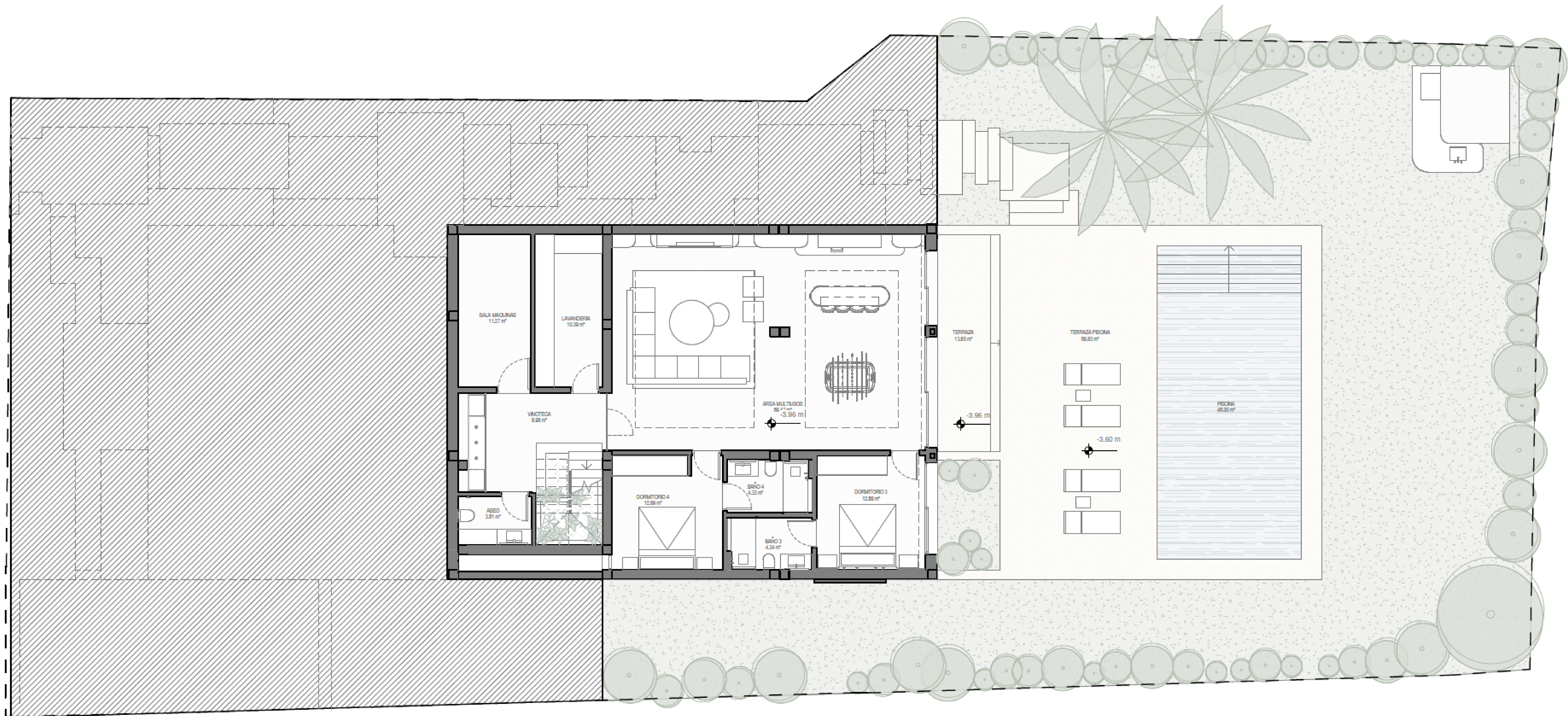
PLANTA SOTANO LOWER LEVEL
