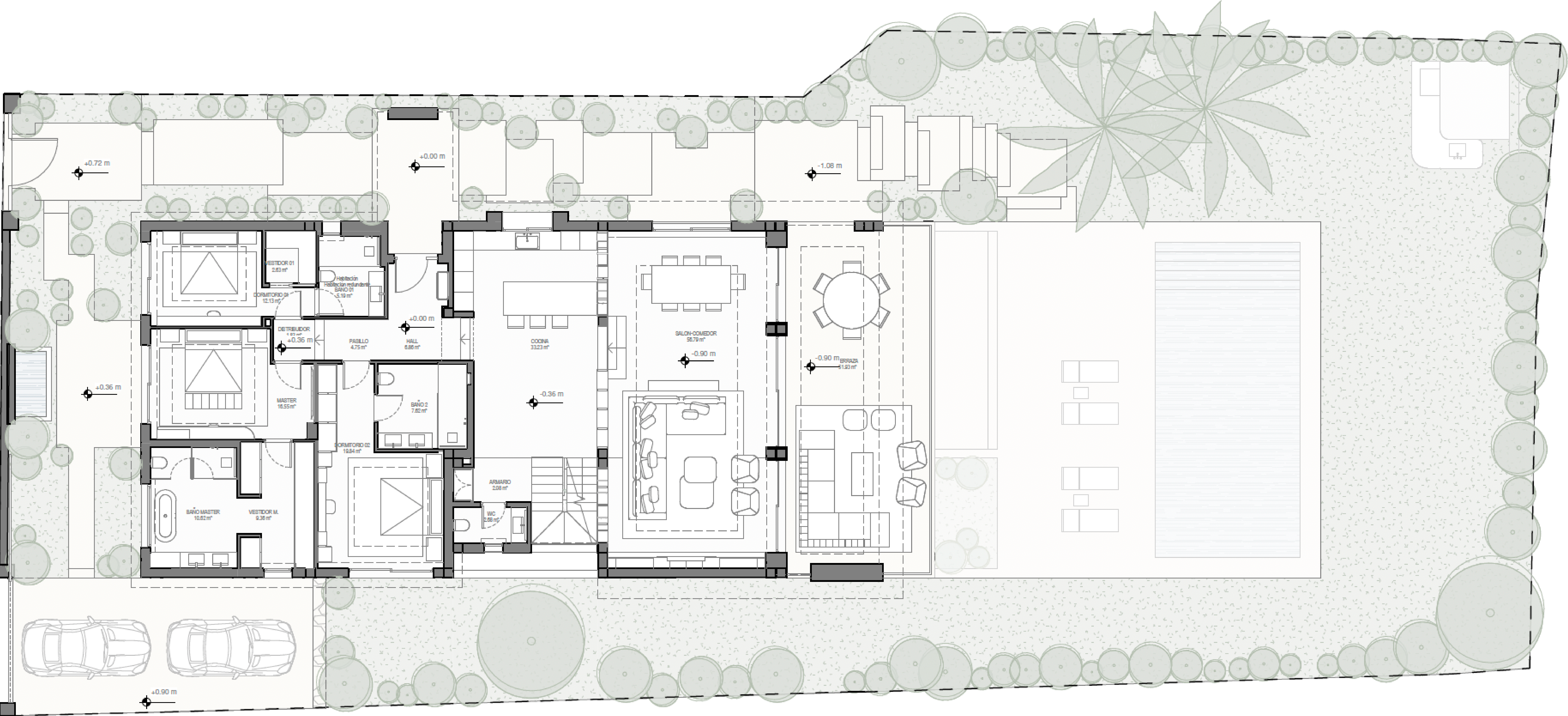
PLANTA BAJA GROUND FLOOR
