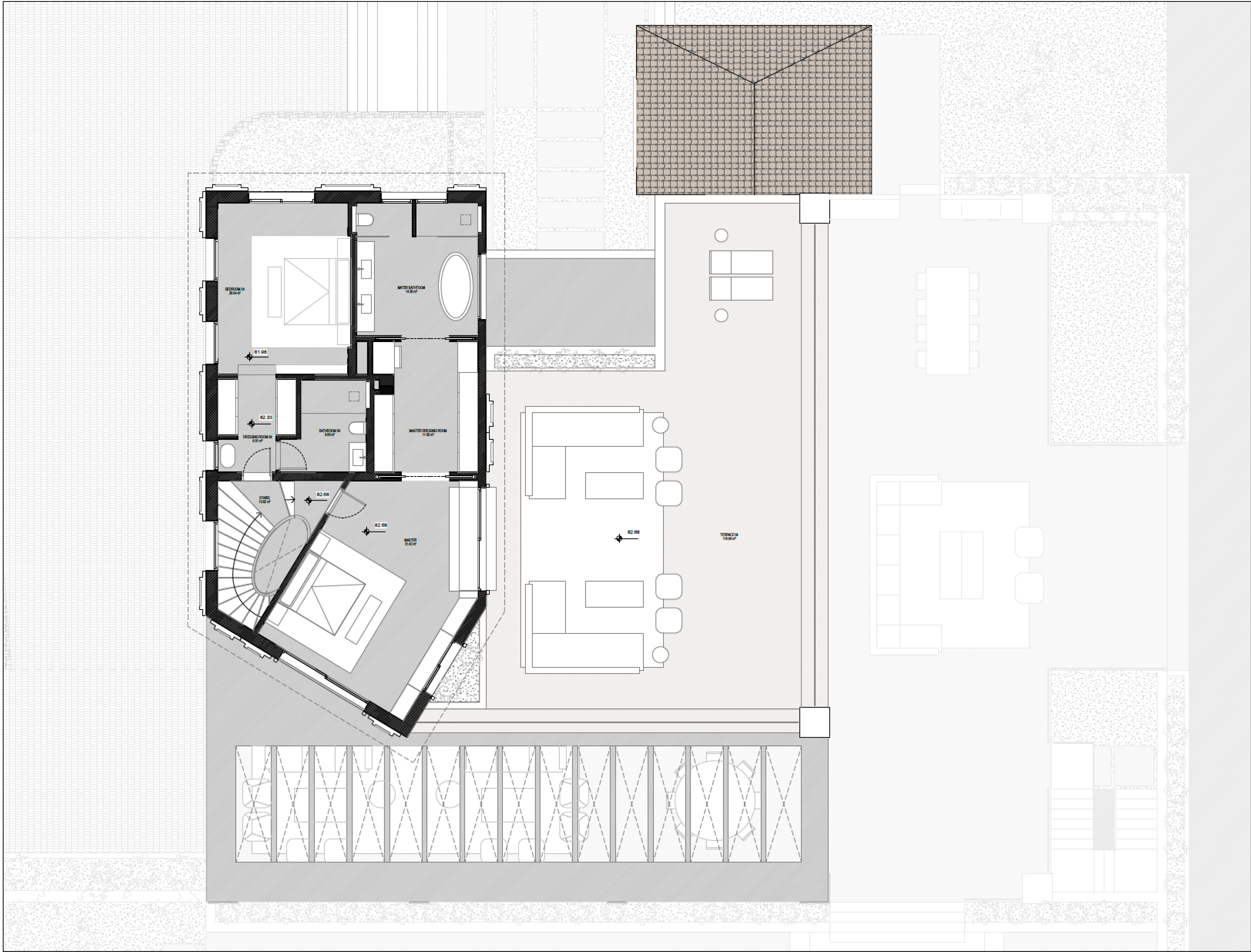
FIRST FLOOR
