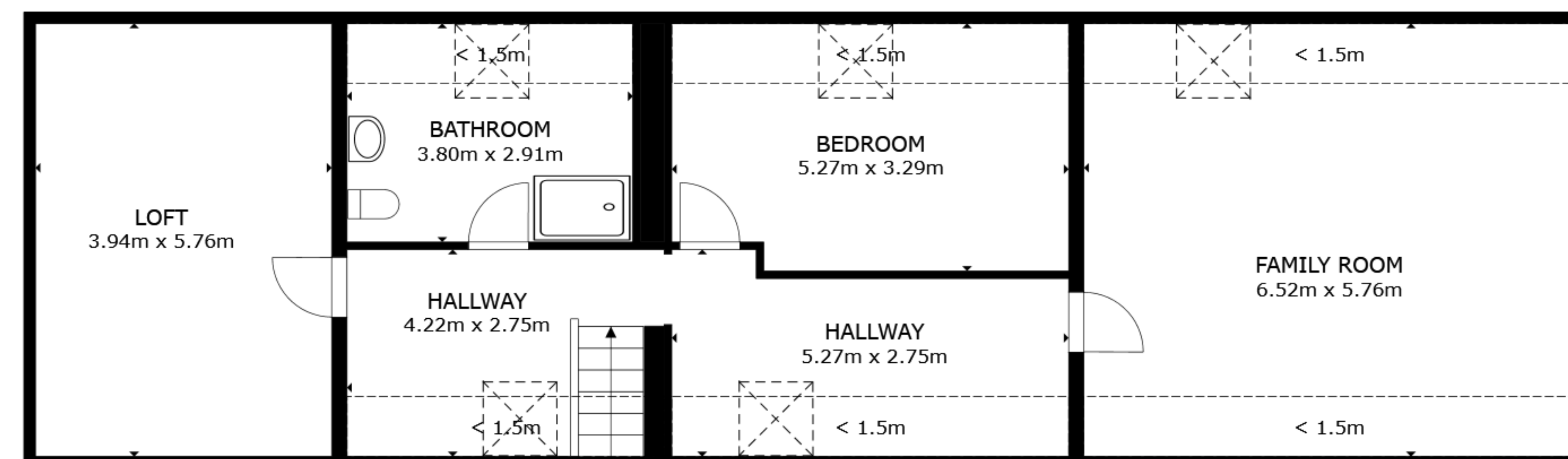
FLOOR 3
