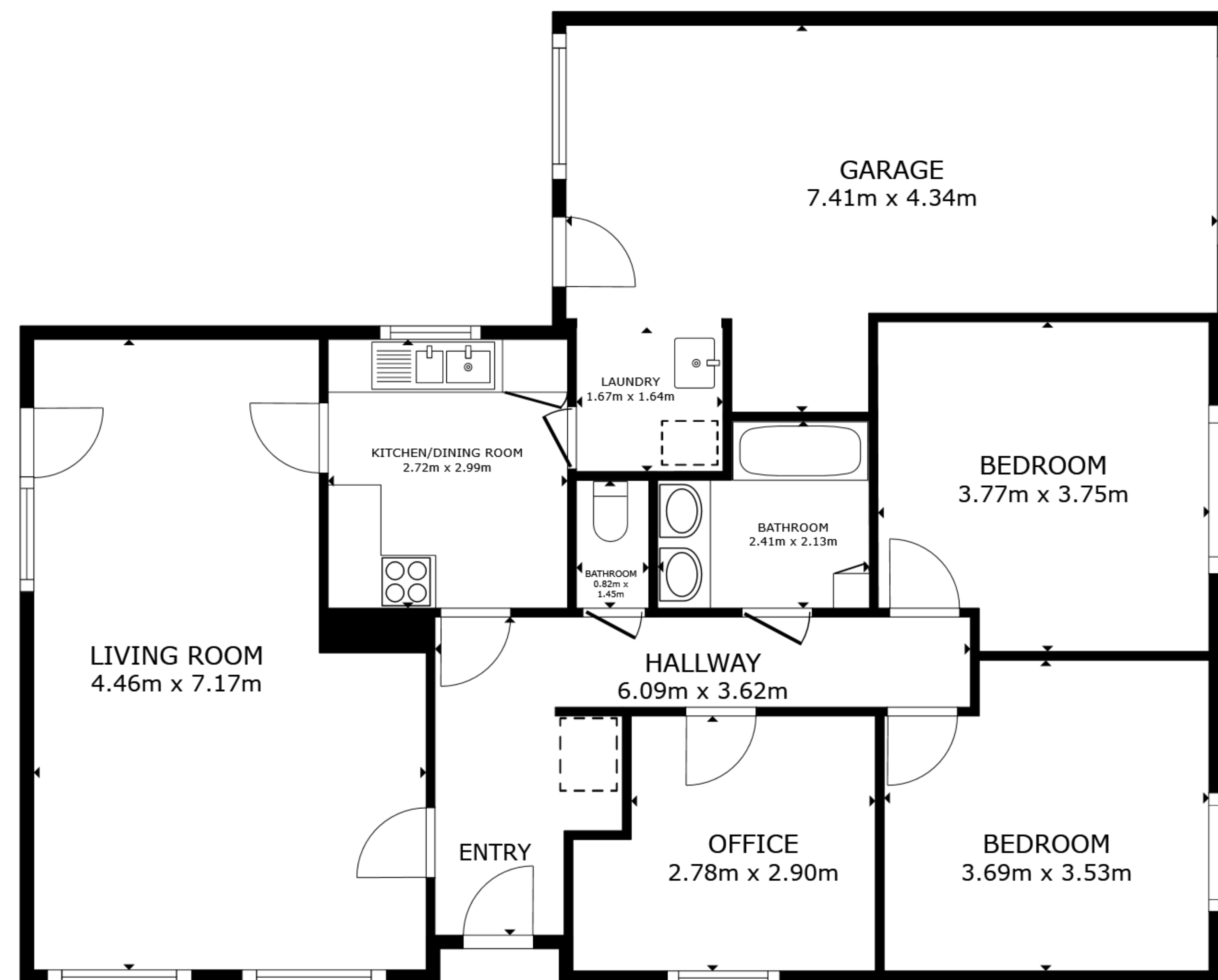
FLOOR PLAN
