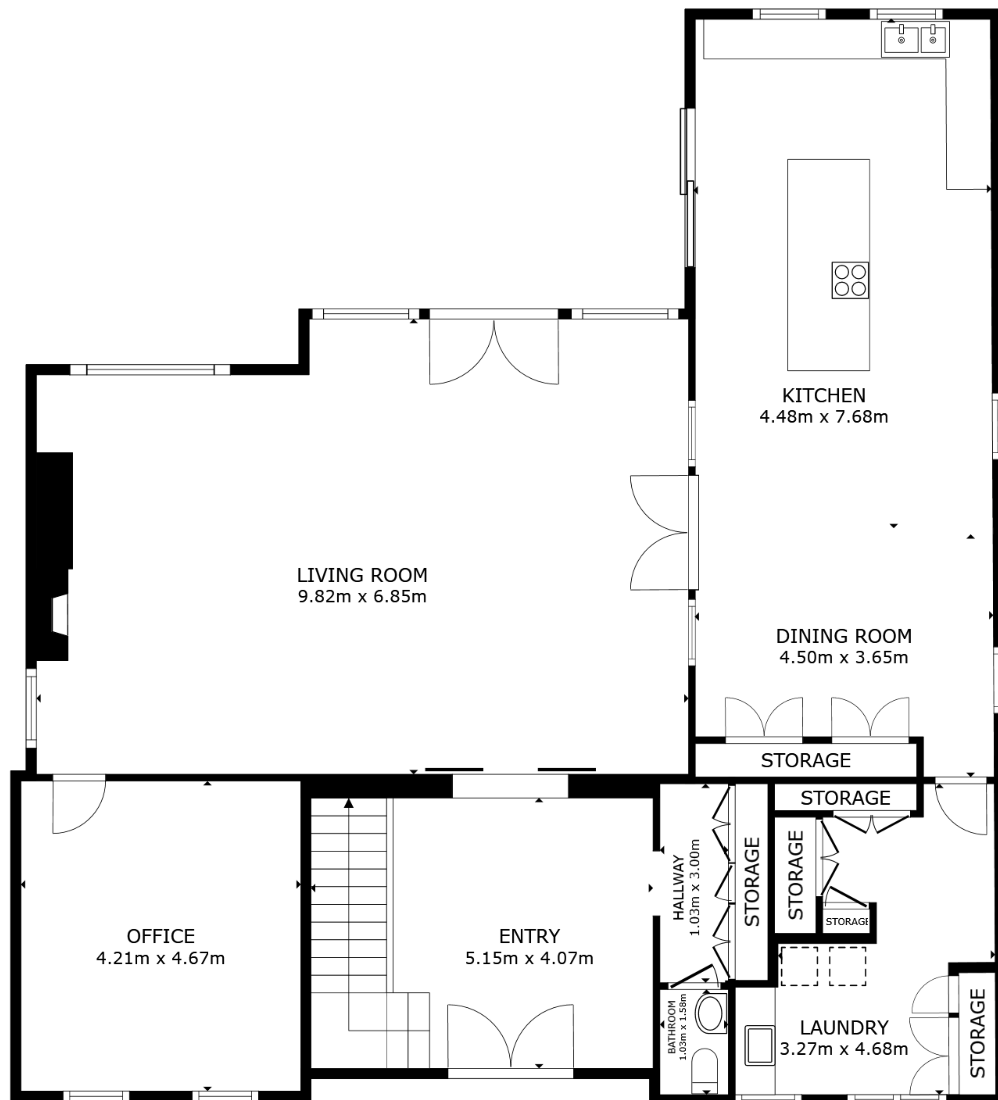
FLOOR 1
