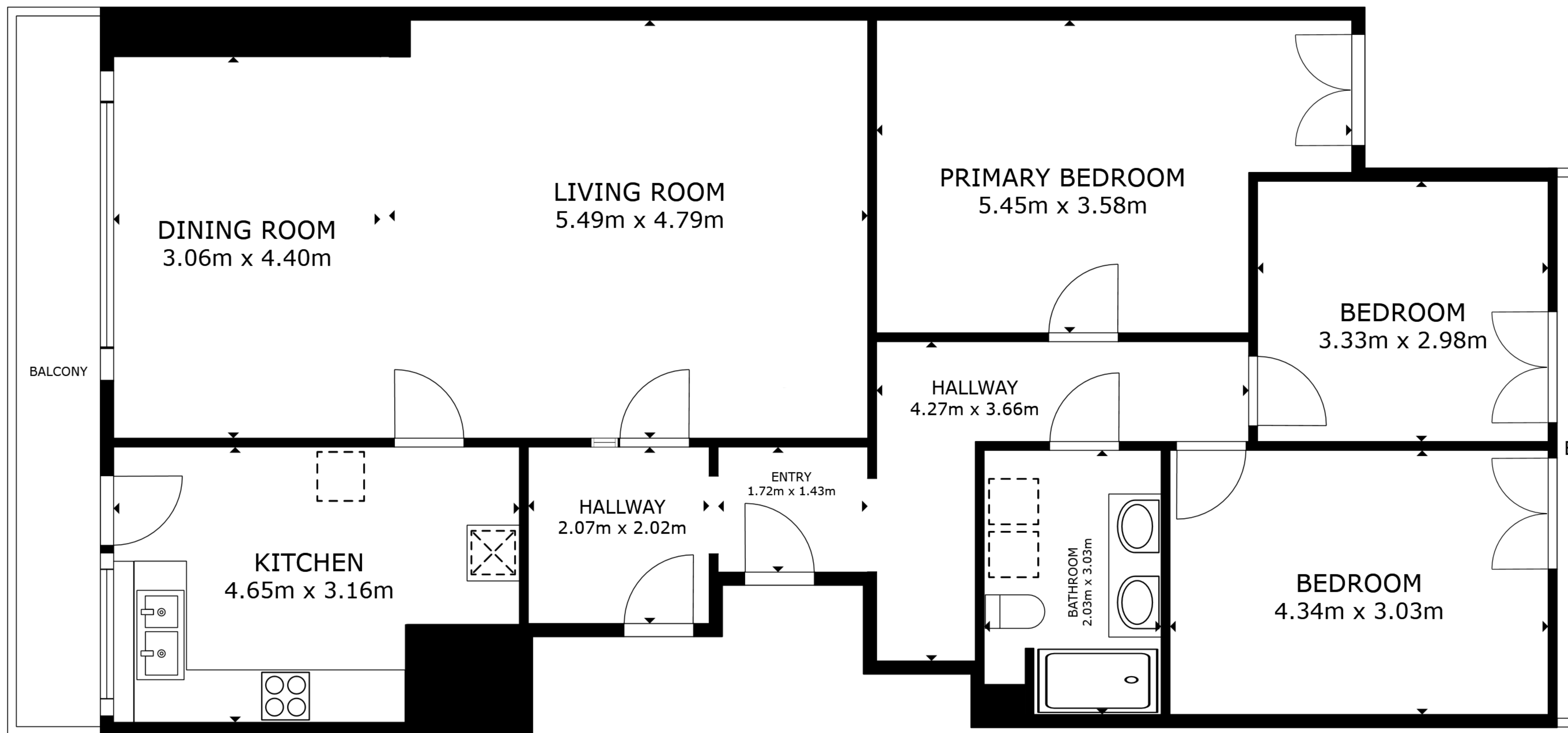
FLOOR PLAN
