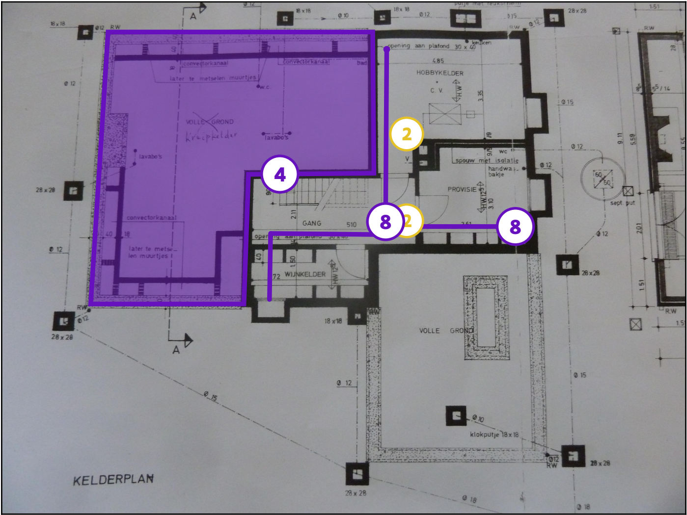
Legende van plan 1.6: Plan nivo -1
