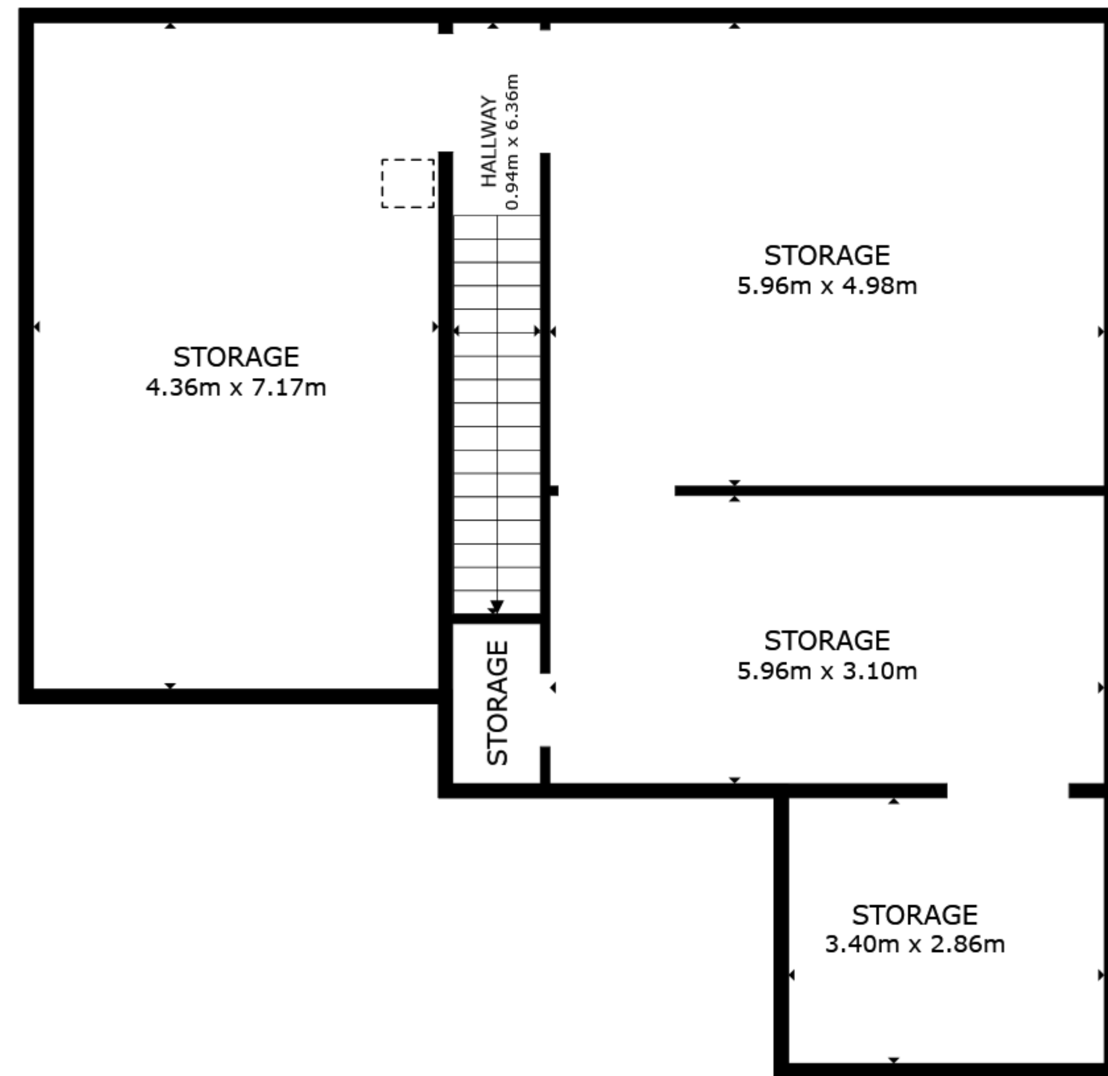
FLOOR 1
