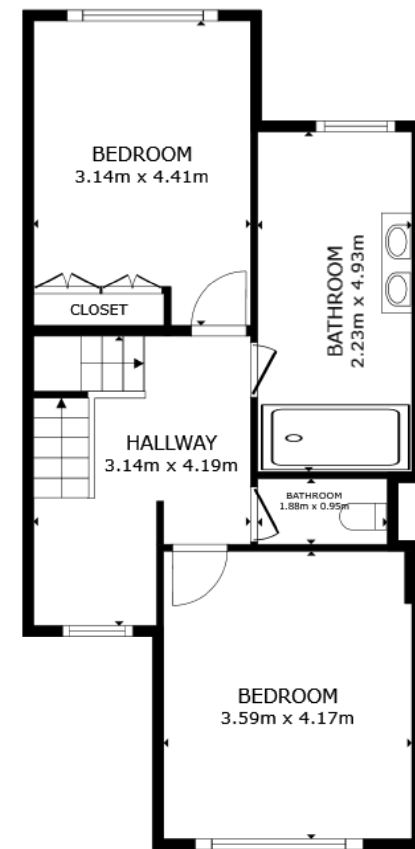
FLOOR 2
