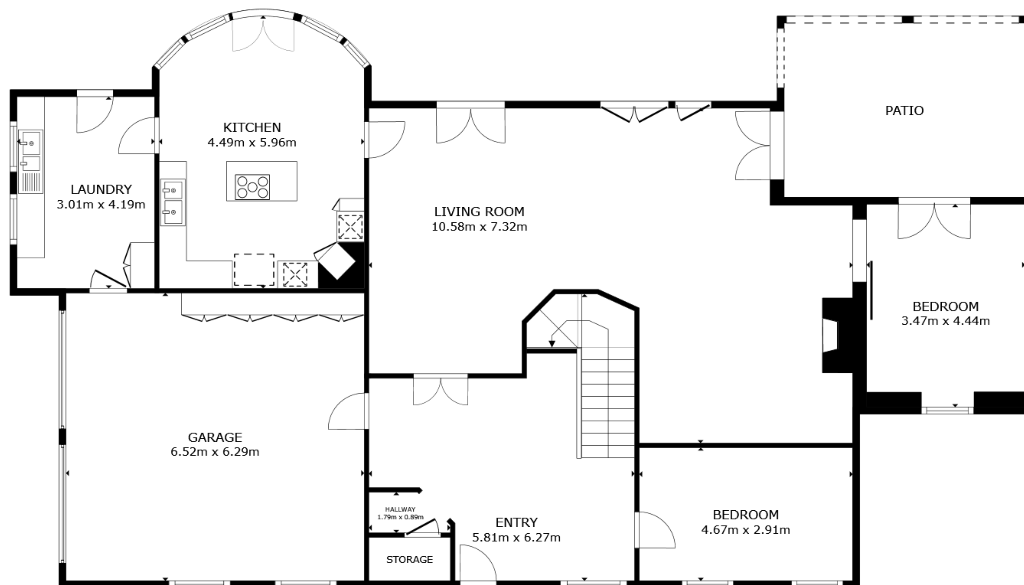
FLOOR 1
