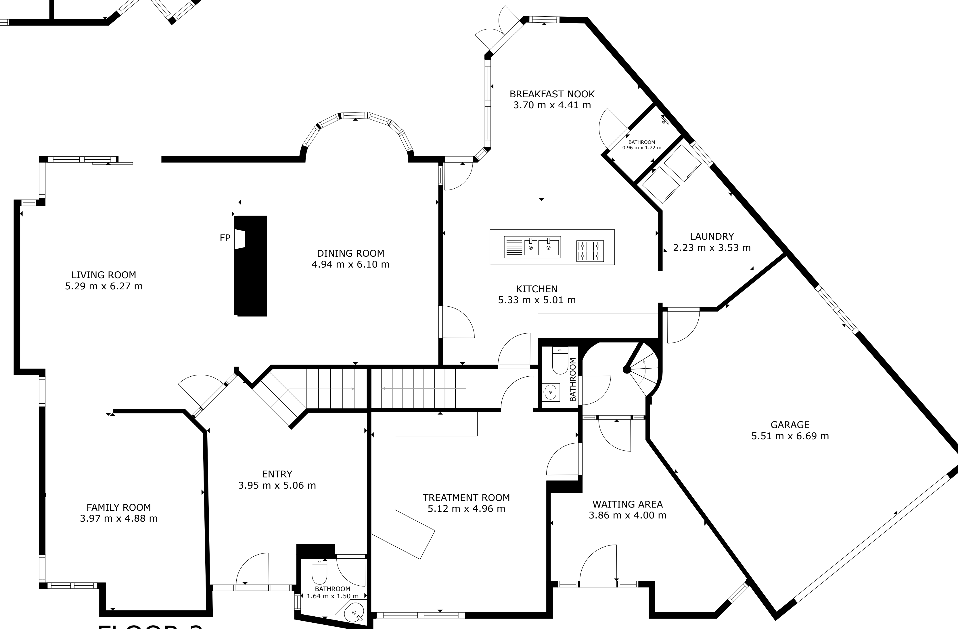
FLOOR 2
