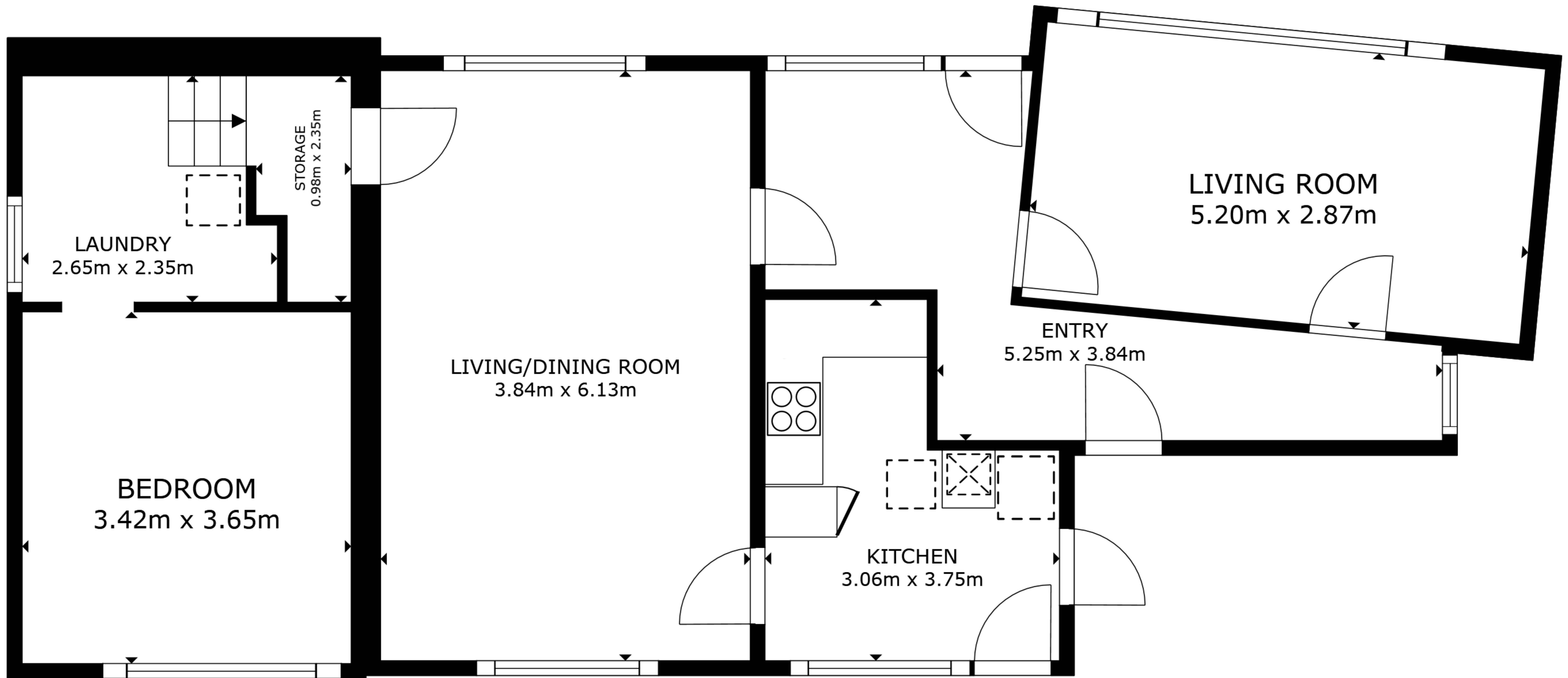
FLOOR PLAN
