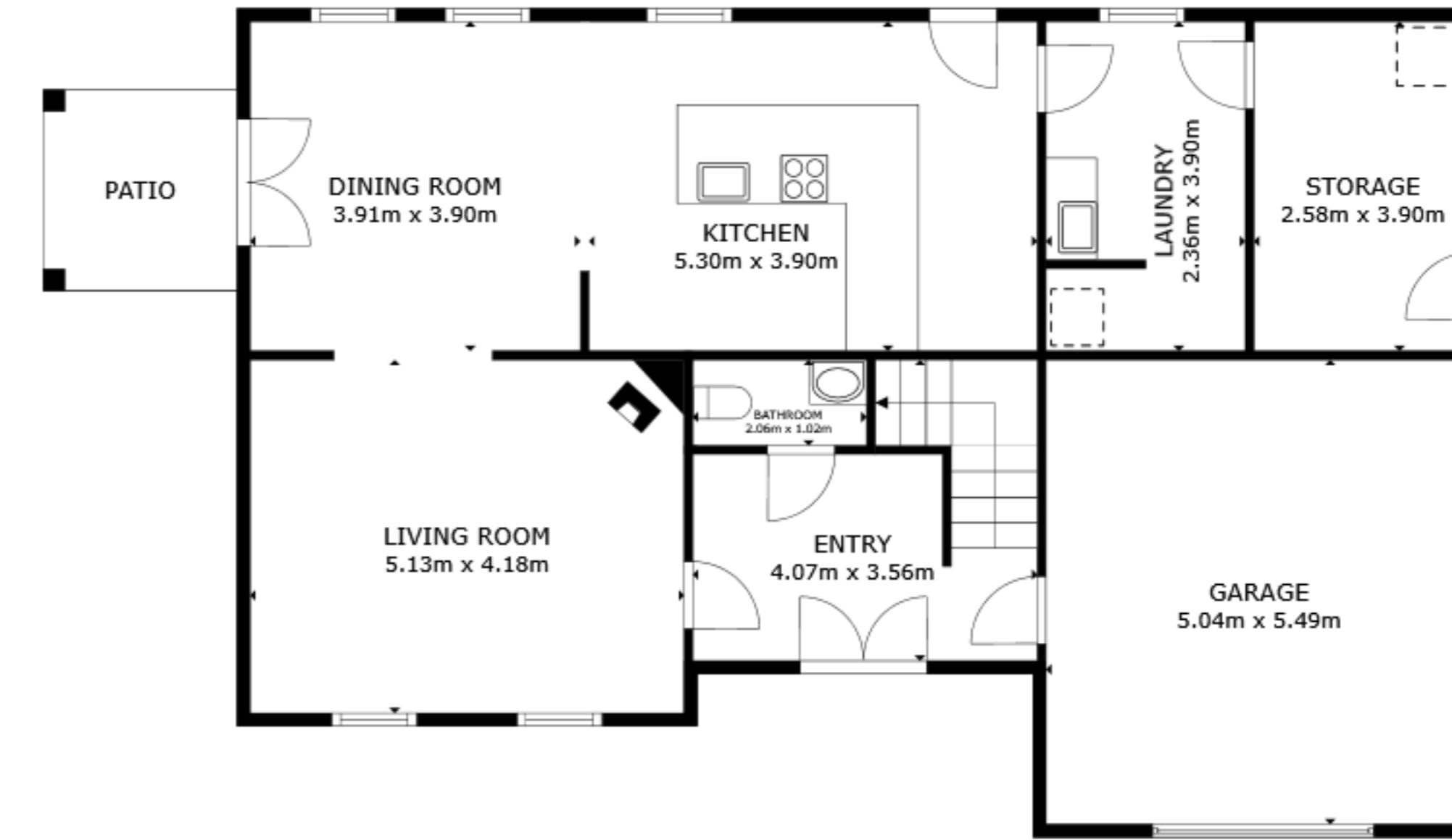
FLOOR 1
