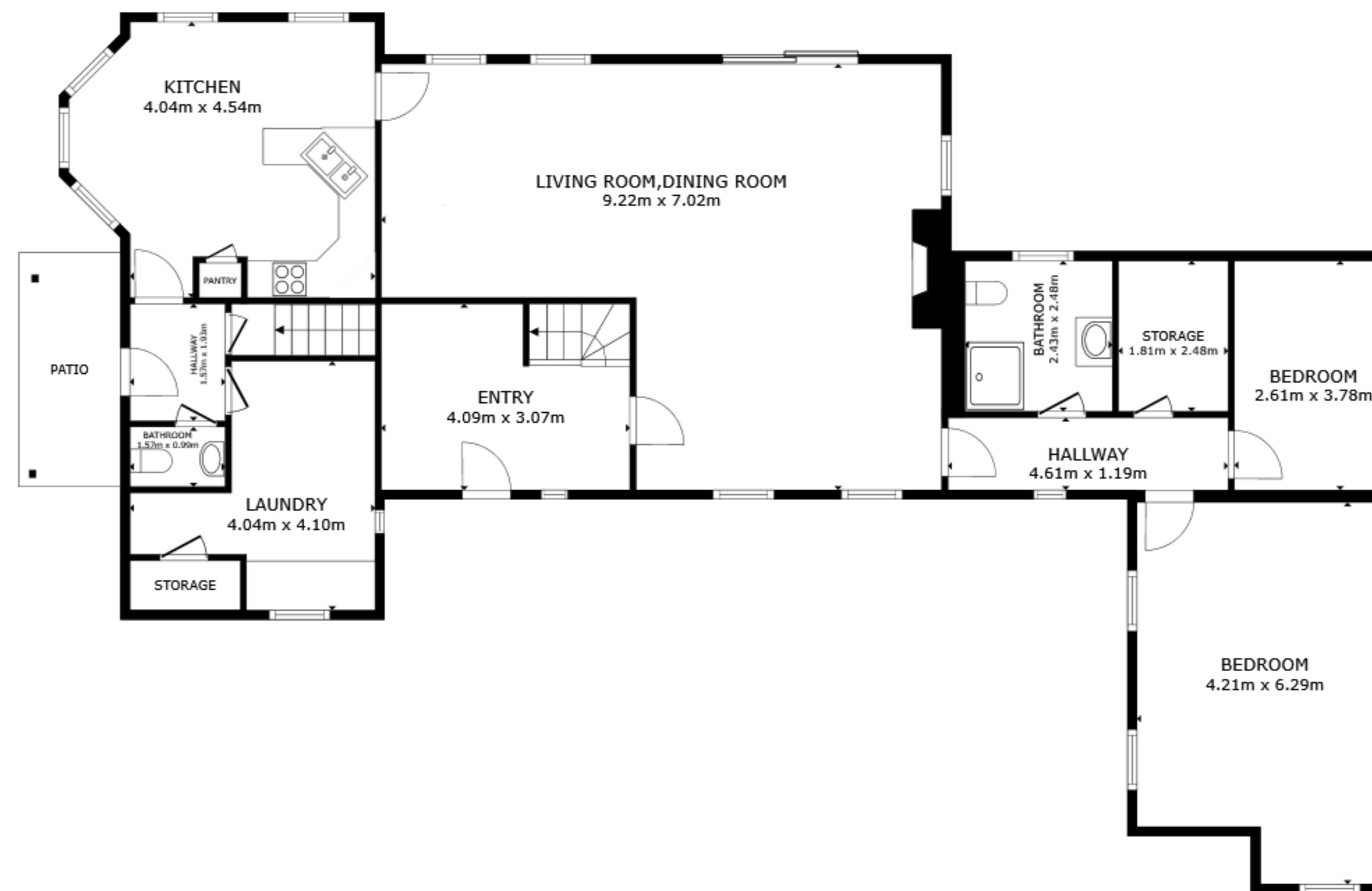
FLOOR 1
