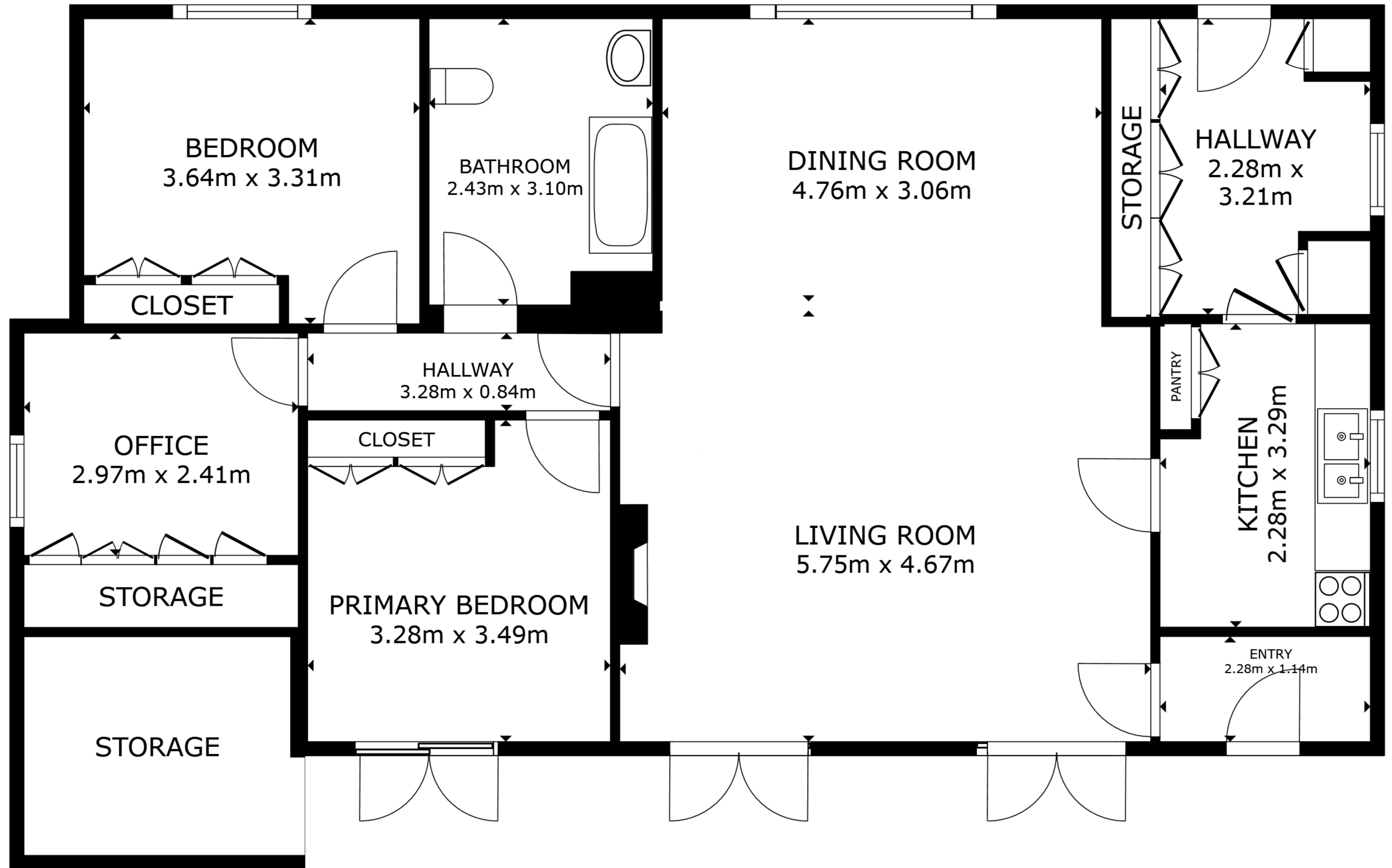
FLOOR PLAN
