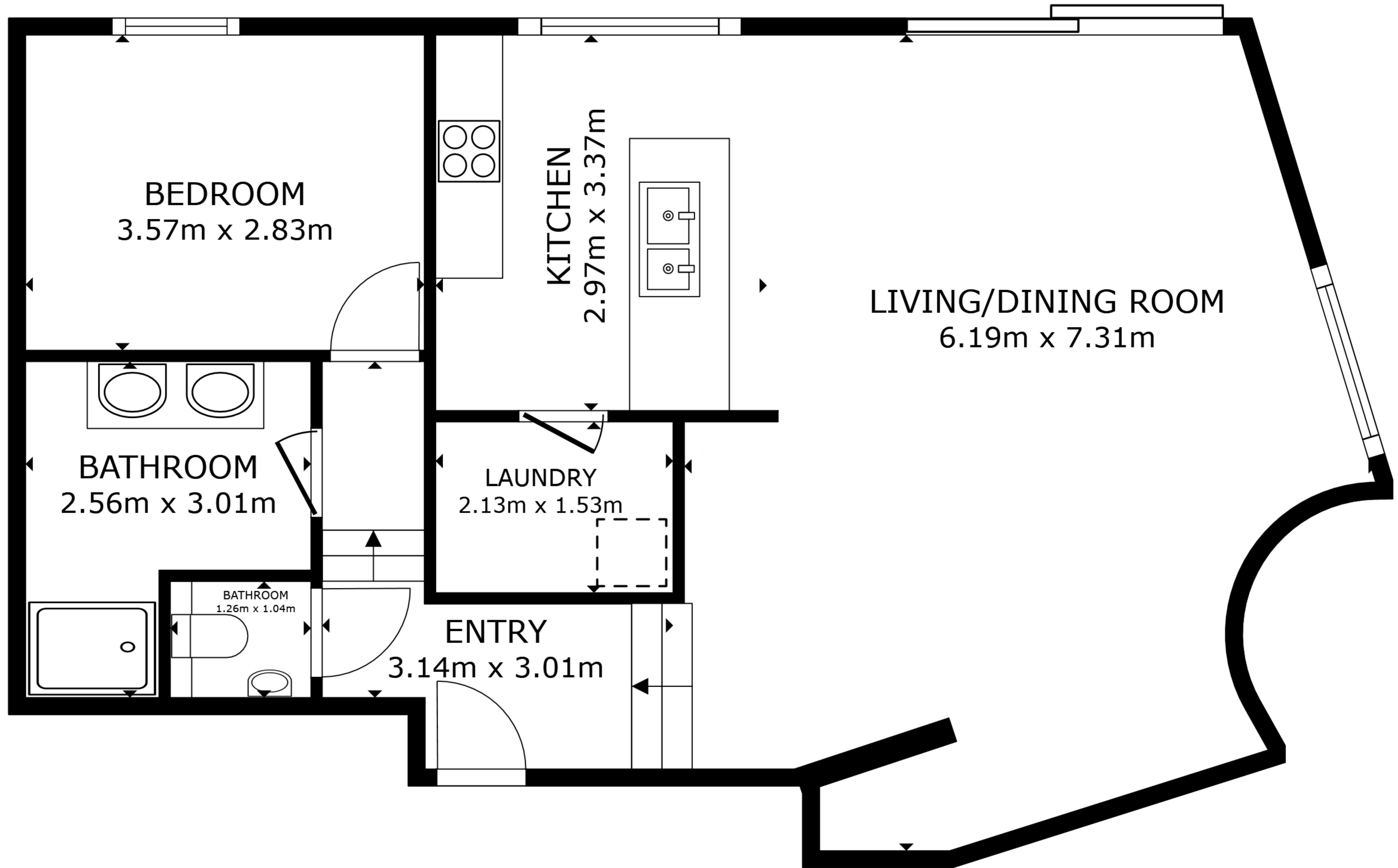
FLOOR PLAN
