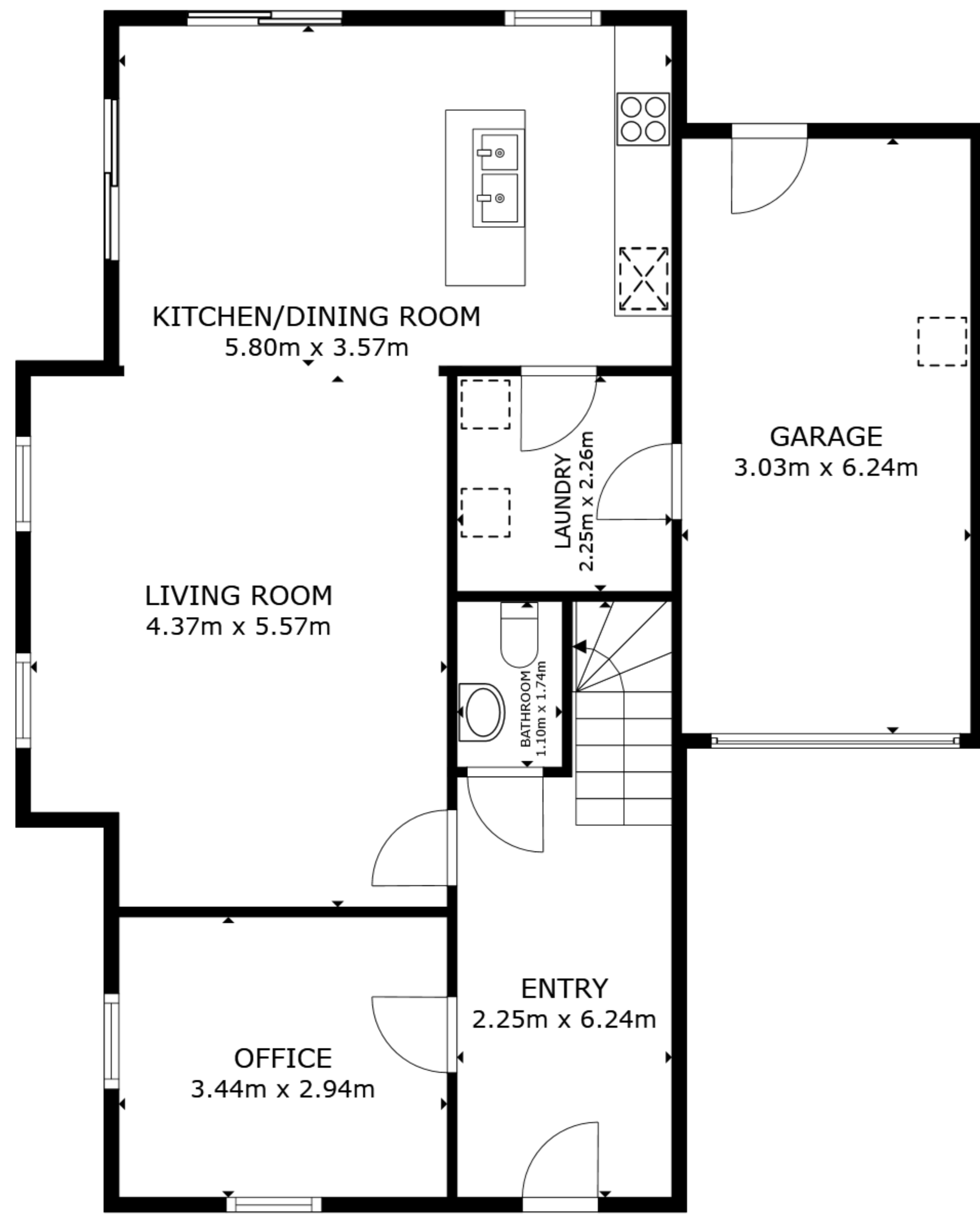
FLOOR 1
