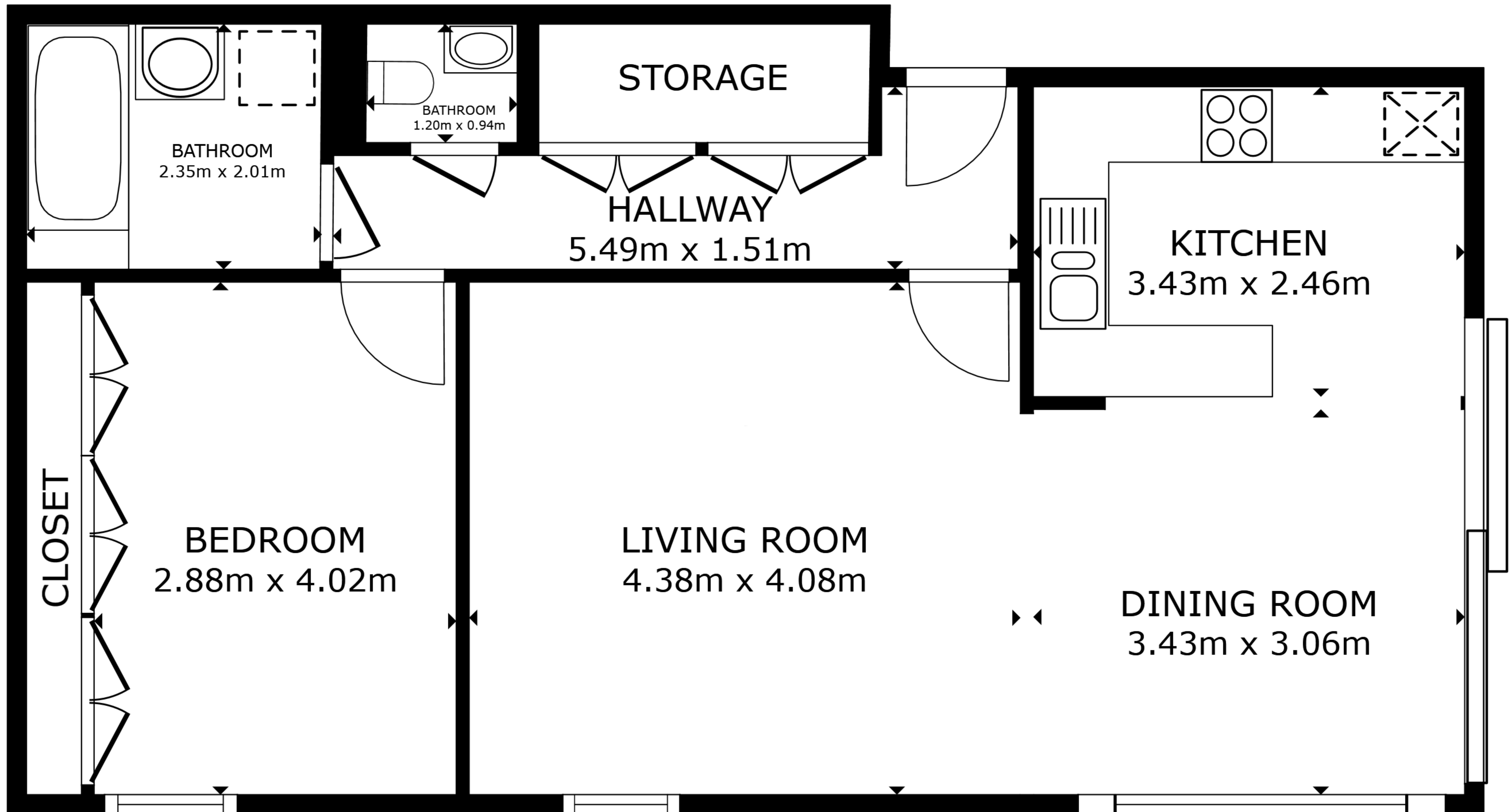
FLOOR PLAN
