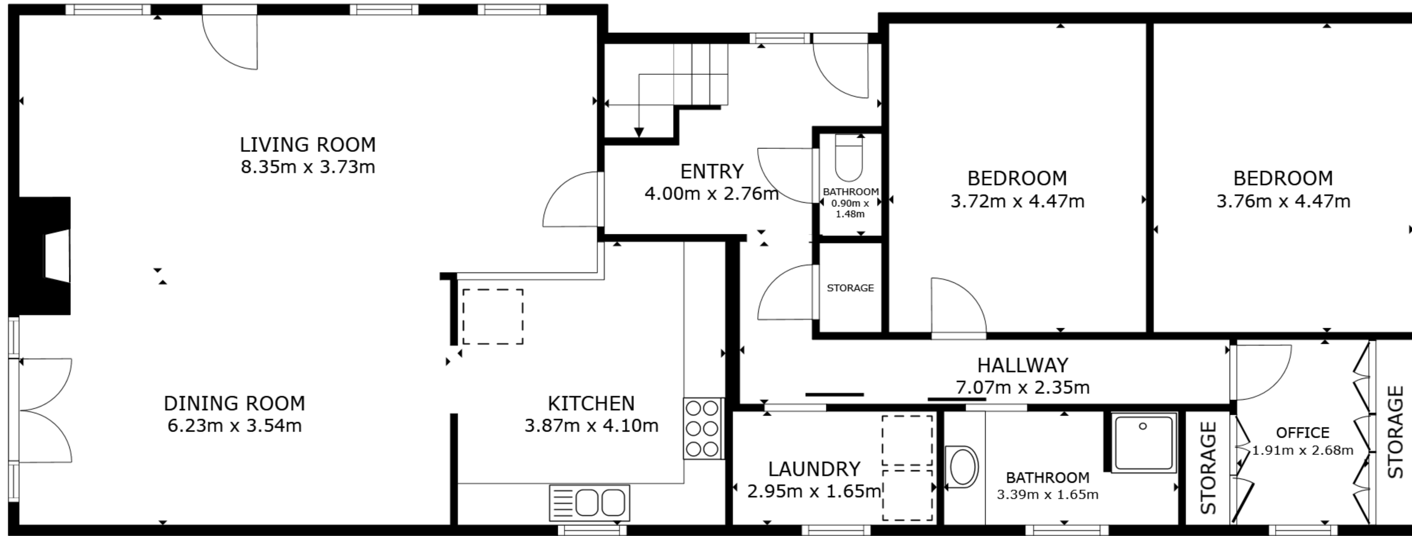
FLOOR 1
