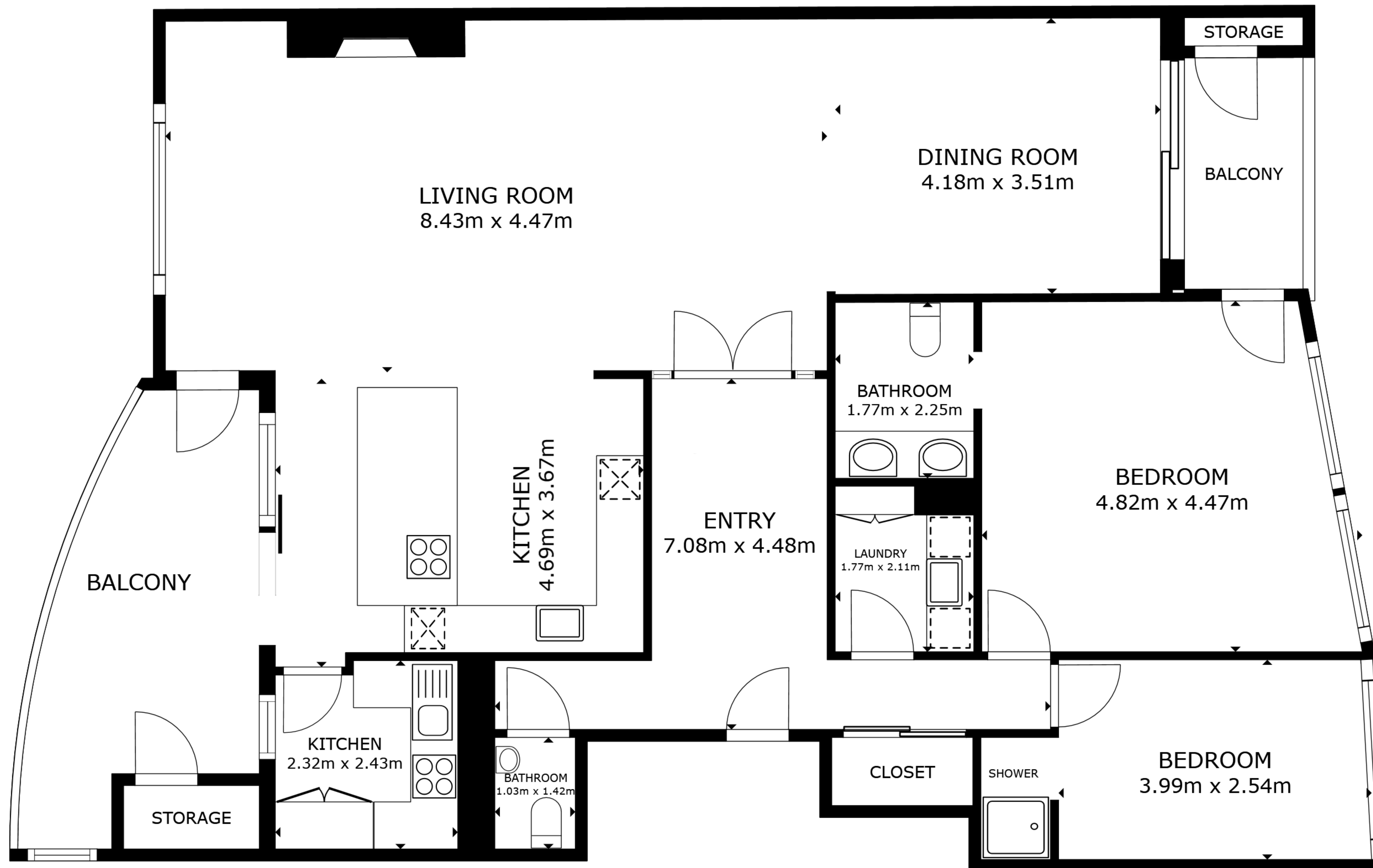
FLOOR PLAN
