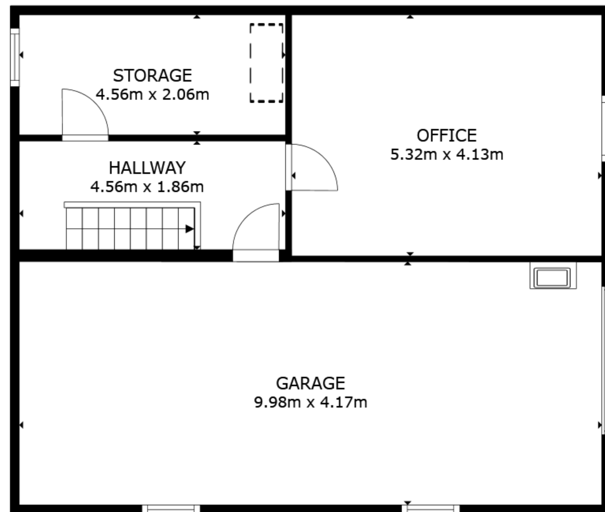
FLOOR 1
