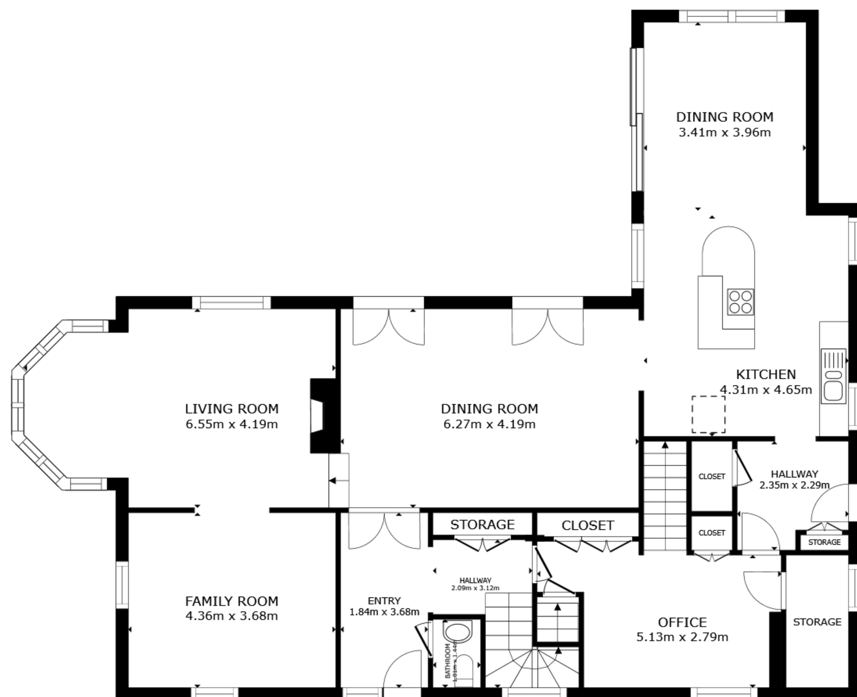
FLOOR 1
