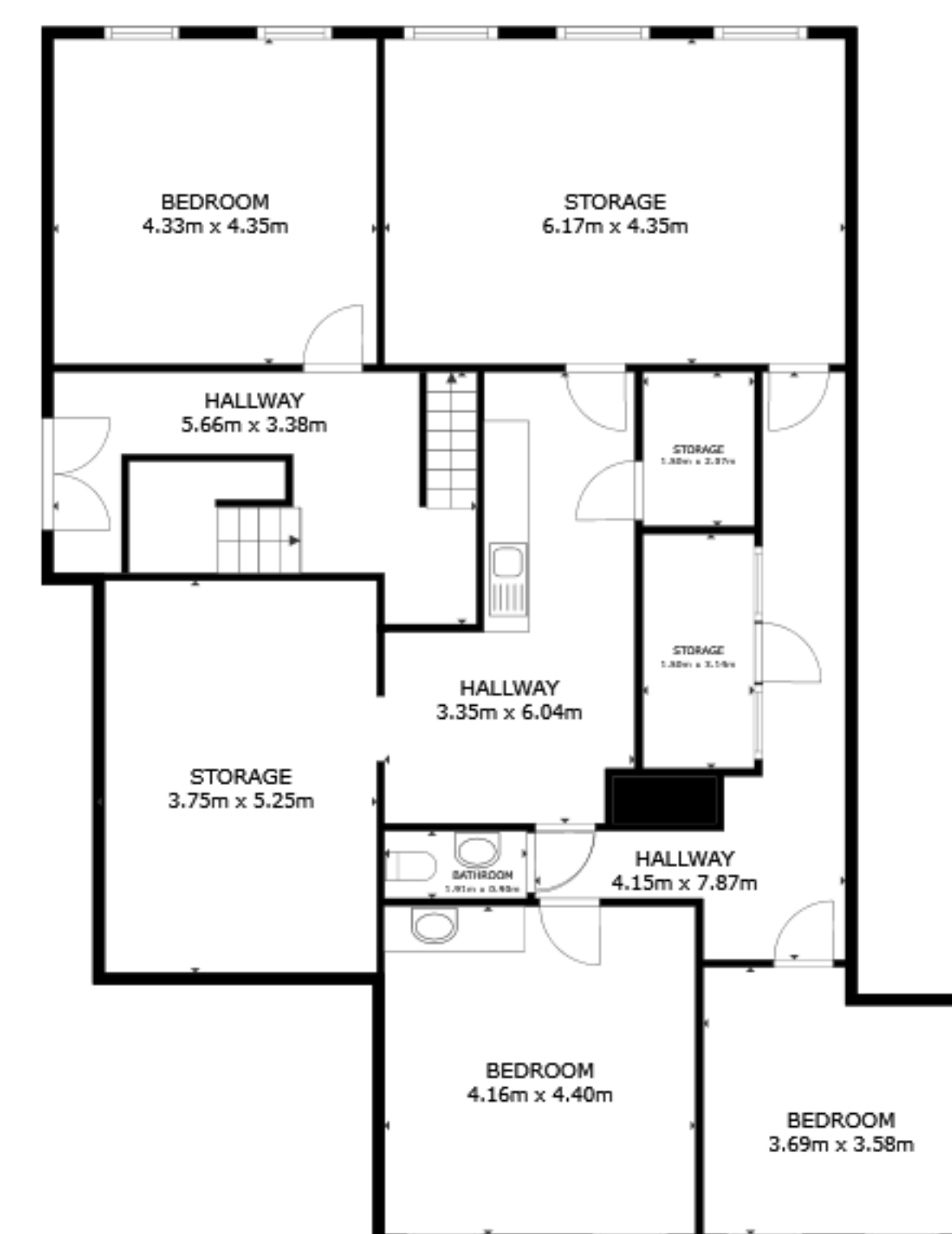
FLOOR 3
