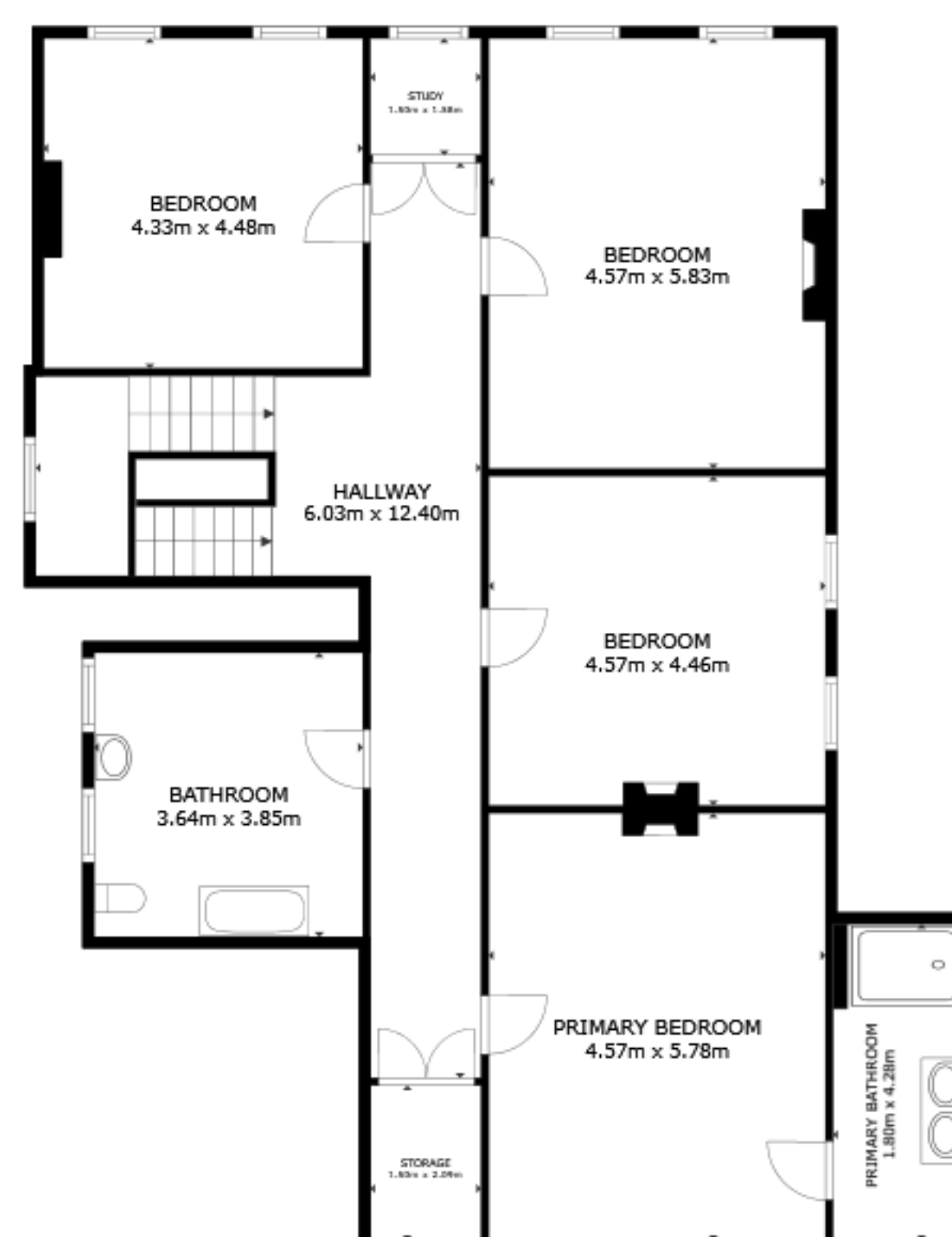
FLOOR 2
