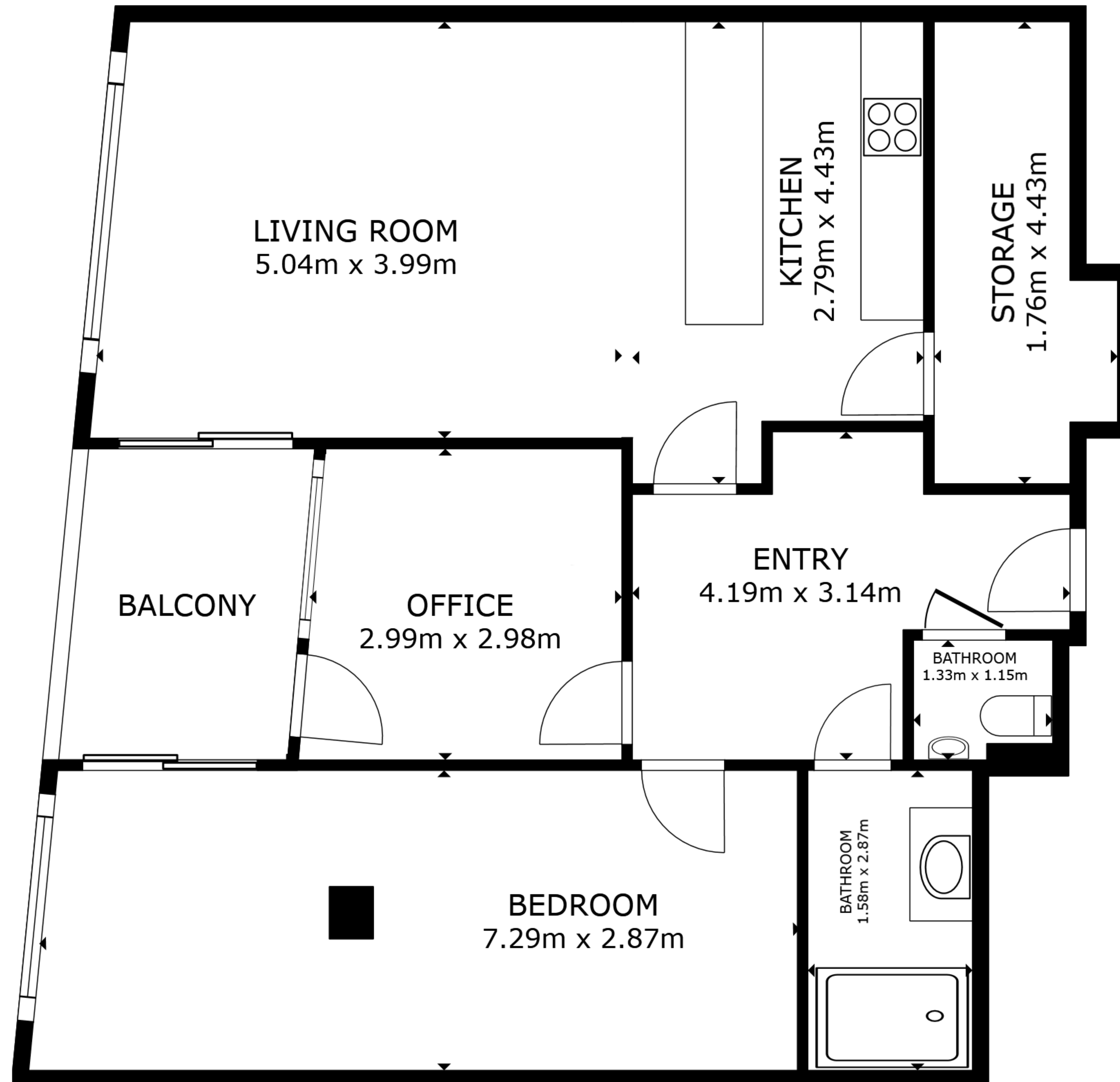
FLOOR PLAN
