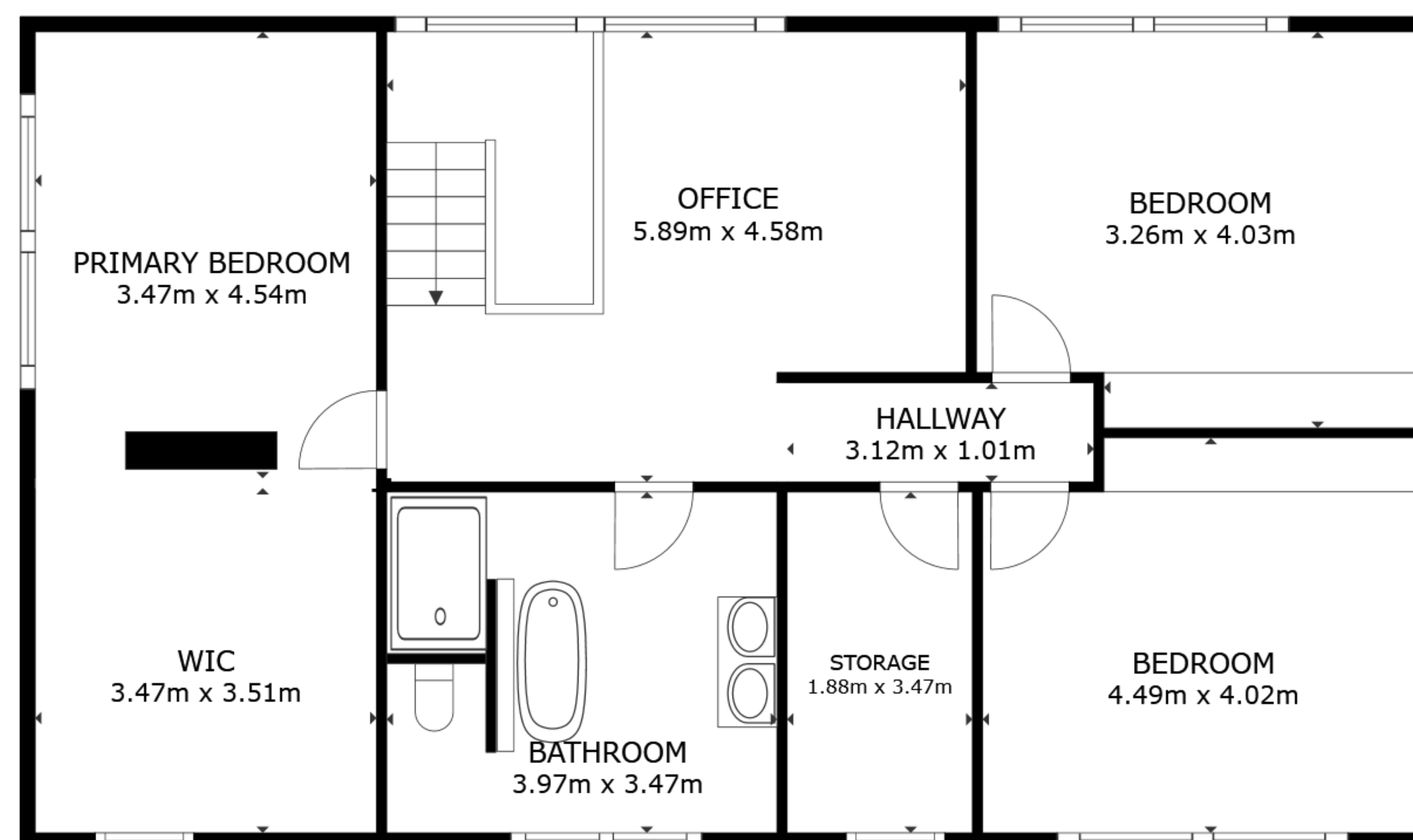
FLOOR 2
