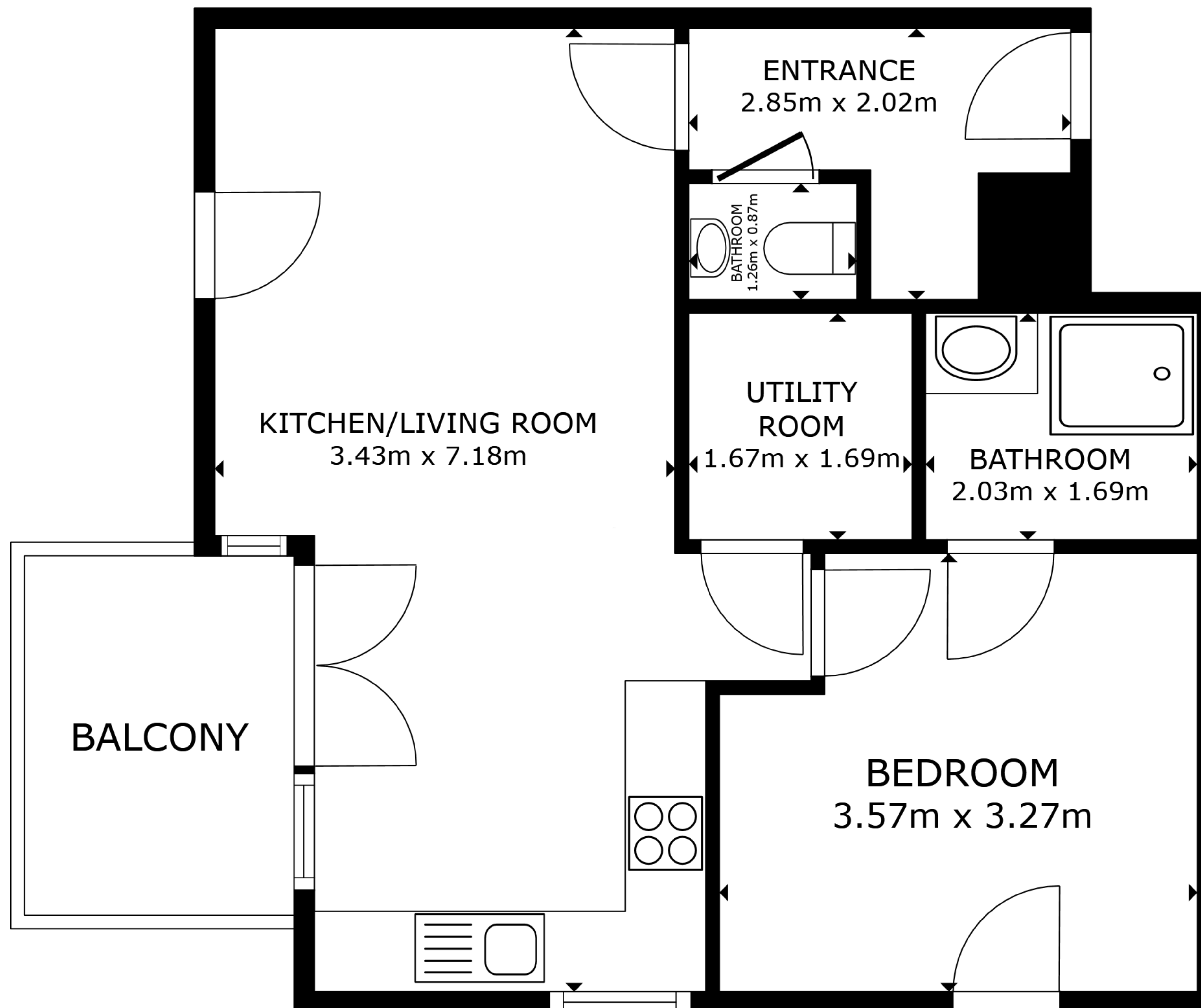
FLOOR PLAN
