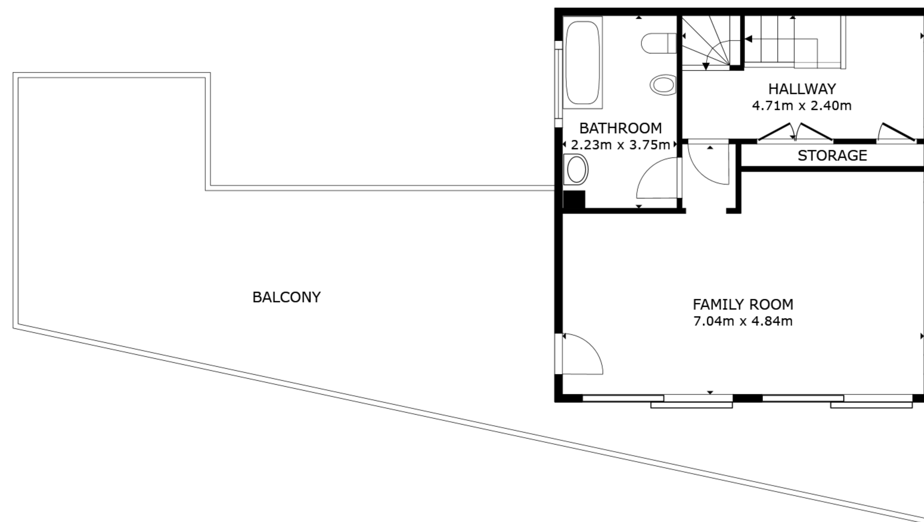
FLOOR 2
