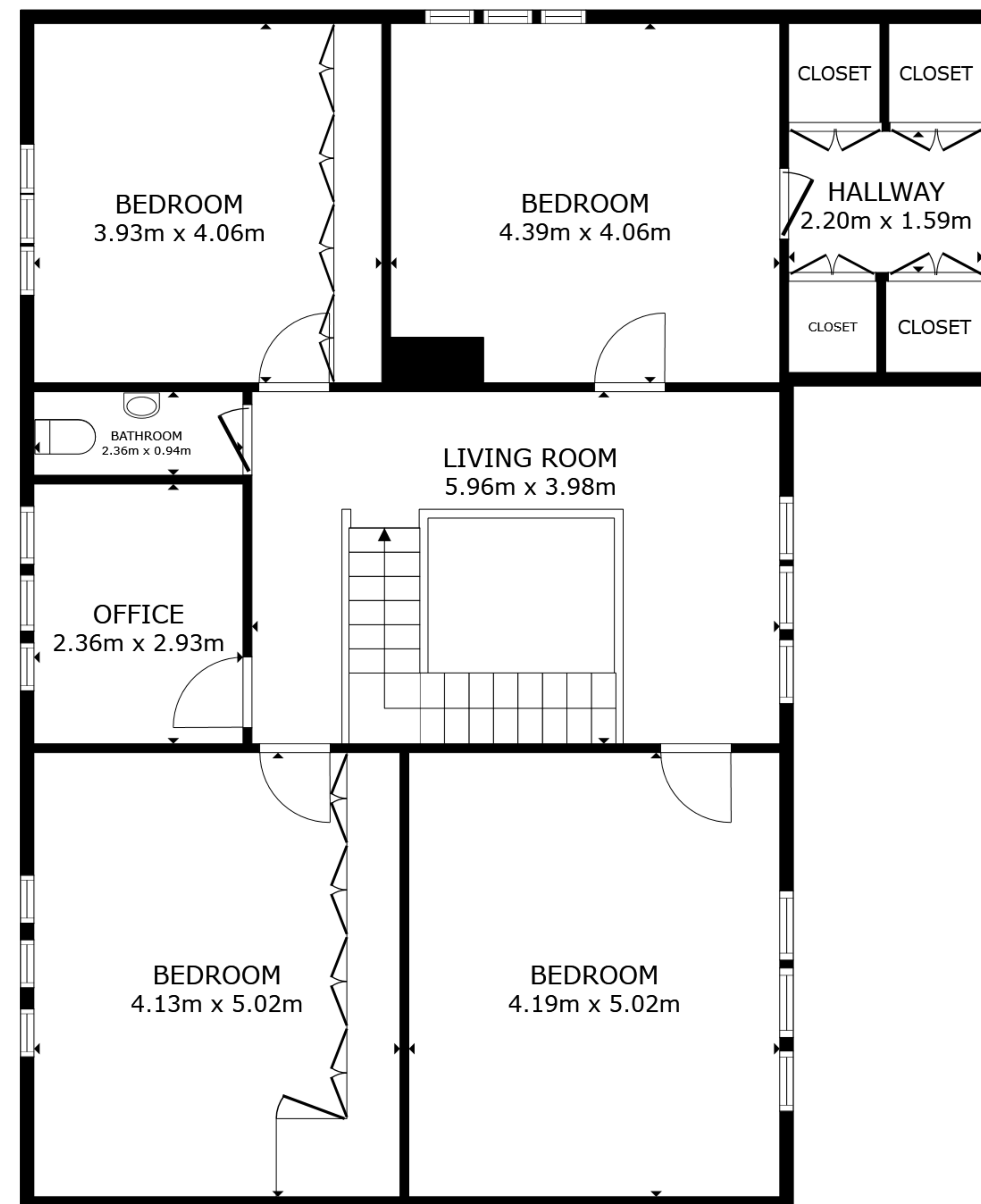
FLOOR 2
